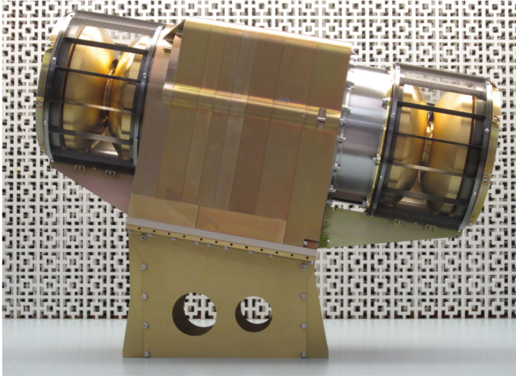
Figure 1. from The Solar Probe ANalyzers—Electrons on the Parker Solar Probe null 2020 APJS 246 74 doi:10.3847/1538-4365/ab7370 https://dx.doi.org/10.3847/1538-4365/ab7370 © 2020. The Author(s). Published by the American Astronomical Society.
