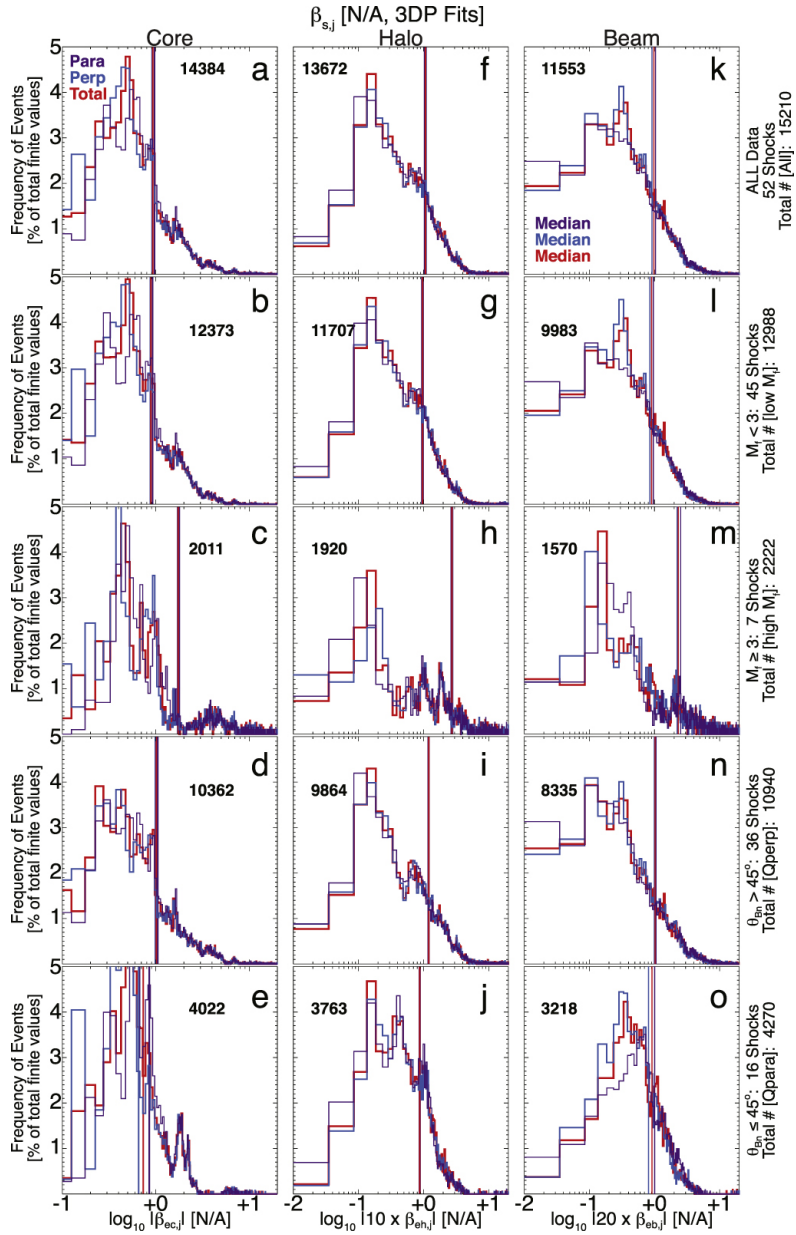
Figure 9. from Electron Energy Partition across Interplanetary Shocks. II. Statistics null 2019 APJS 245 24 doi:10.3847/1538-4365/ab5445 https://dx.doi.org/10.3847/1538-4365/ab5445 © 2019. The American Astronomical Society.
