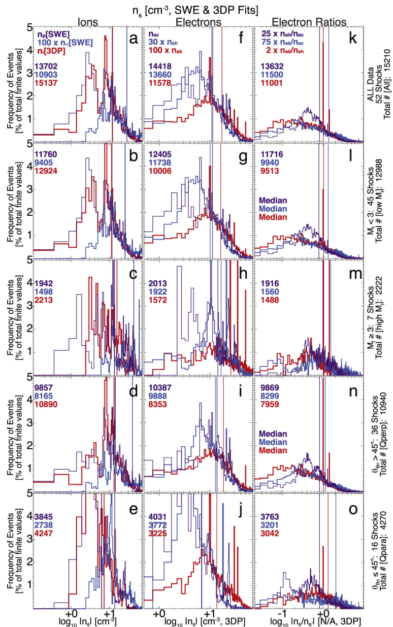
Figure 8. from Electron Energy Partition across Interplanetary Shocks. II. Statistics null 2019 APJS 245 24 doi:10.3847/1538-4365/ab5445 https://dx.doi.org/10.3847/1538-4365/ab5445 © 2019. The American Astronomical Society.
