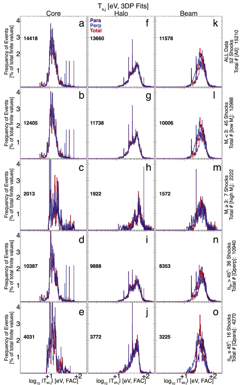
Figure 7. from Electron Energy Partition across Interplanetary Shocks. II. Statistics null 2019 APJS 245 24 doi:10.3847/1538-4365/ab5445 https://dx.doi.org/10.3847/1538-4365/ab5445 © 2019. The American Astronomical Society.
