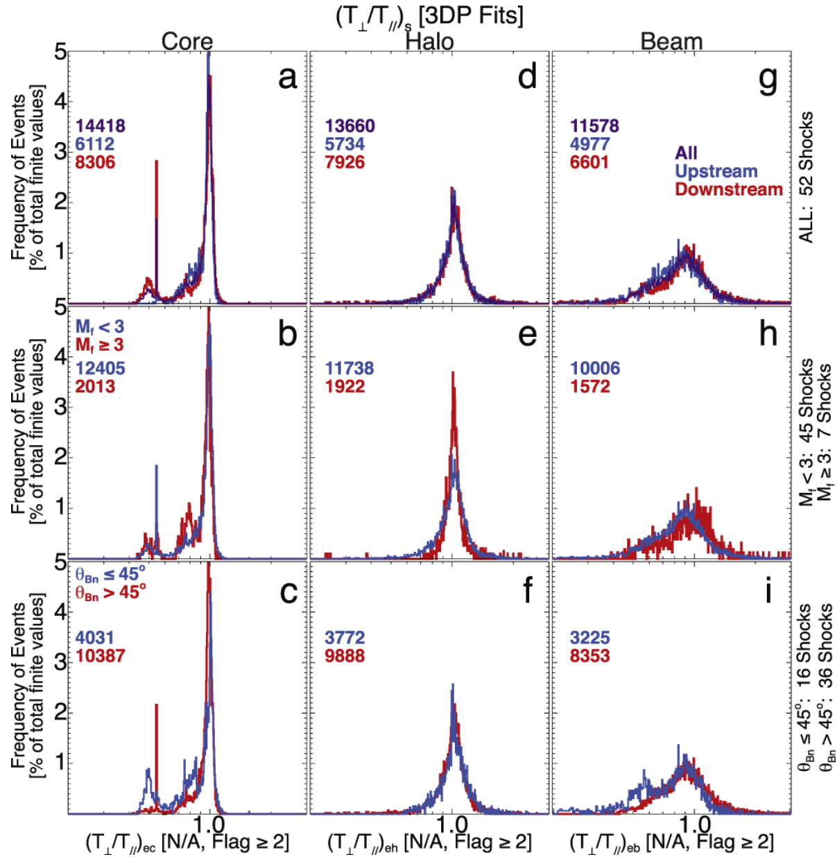
Figure 5. from Electron Energy Partition across Interplanetary Shocks. II. Statistics null 2019 APJS 245 24 doi:10.3847/1538-4365/ab5445 https://dx.doi.org/10.3847/1538-4365/ab5445 © 2019. The American Astronomical Society.
