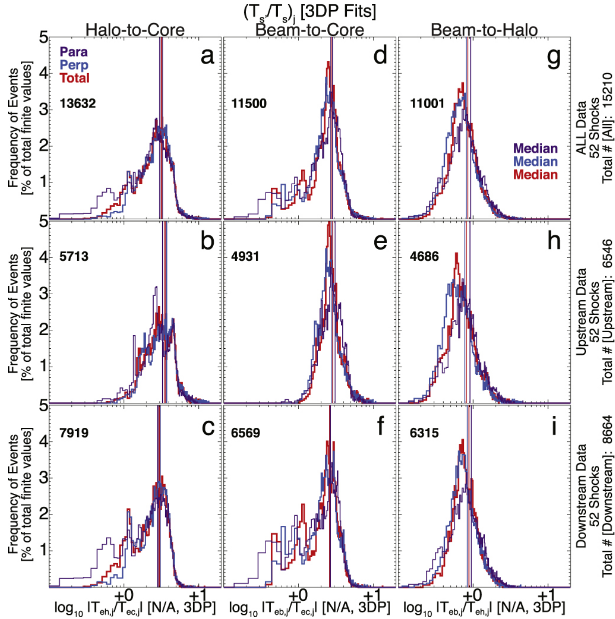
Figure 4. from Electron Energy Partition across Interplanetary Shocks. II. Statistics null 2019 APJS 245 24 doi:10.3847/1538-4365/ab5445 https://dx.doi.org/10.3847/1538-4365/ab5445 © 2019. The American Astronomical Society.
