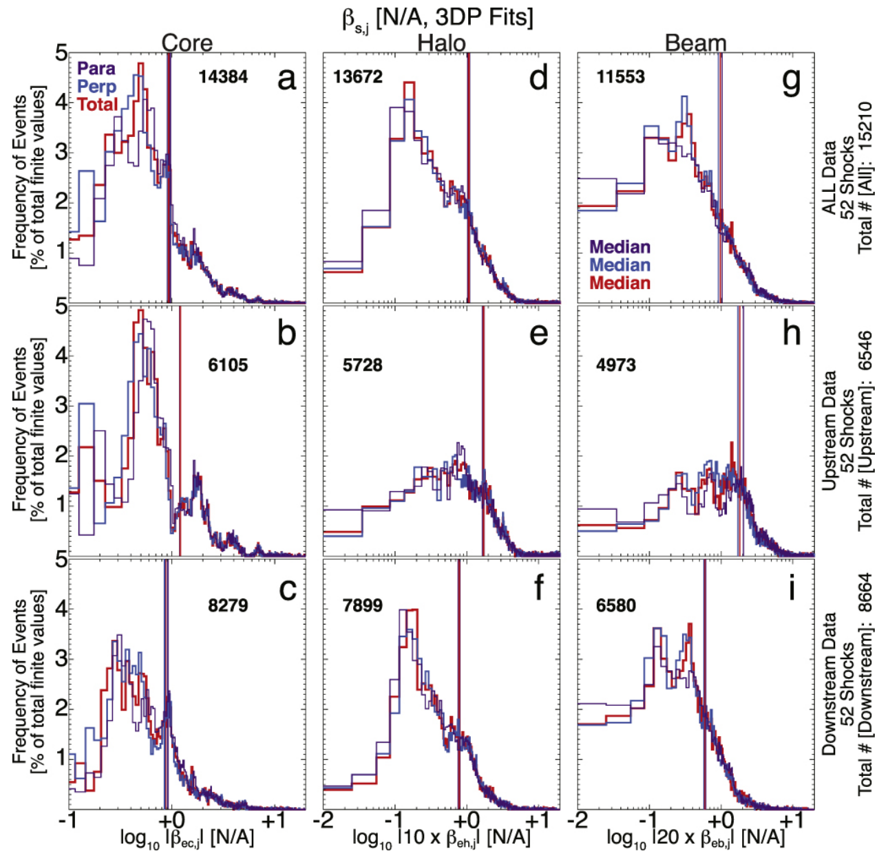
Figure 3. from Electron Energy Partition across Interplanetary Shocks. II. Statistics null 2019 APJS 245 24 doi:10.3847/1538-4365/ab5445 https://dx.doi.org/10.3847/1538-4365/ab5445 © 2019. The American Astronomical Society.
