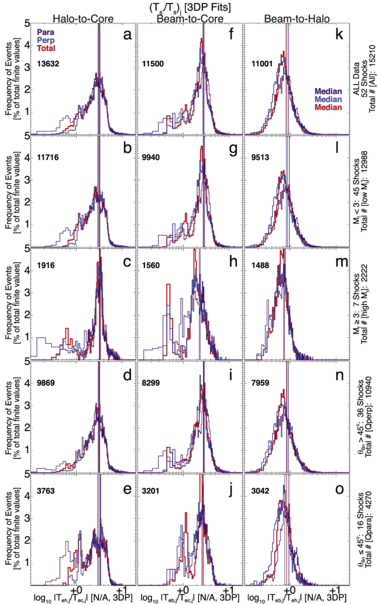
Figure 10. from Electron Energy Partition across Interplanetary Shocks. II. Statistics null 2019 APJS 245 24 doi:10.3847/1538-4365/ab5445 https://dx.doi.org/10.3847/1538-4365/ab5445 © 2019. The American Astronomical Society.
