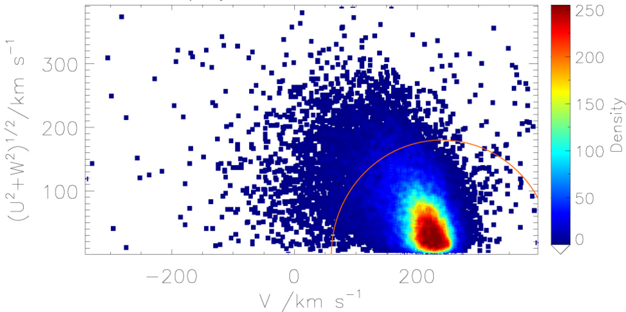
Figure 9. from Value-added Catalogs of M-type Stars in LAMOST DR5 null 2019 APJS 244 8 doi:10.3847/1538-4365/ab3859 https://dx.doi.org/10.3847/1538-4365/ab3859 © 2019. The American Astronomical Society. All rights reserved.
