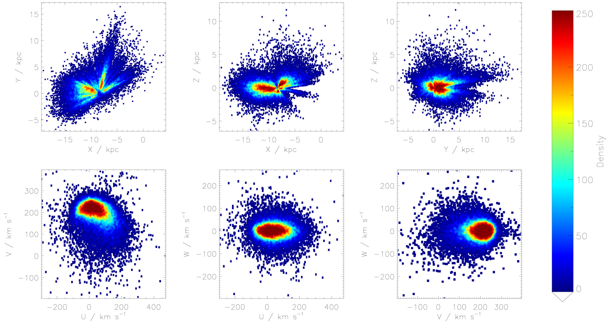
Figure 8. from Value-added Catalogs of M-type Stars in LAMOST DR5 null 2019 APJS 244 8 doi:10.3847/1538-4365/ab3859 https://dx.doi.org/10.3847/1538-4365/ab3859 © 2019. The American Astronomical Society. All rights reserved.
