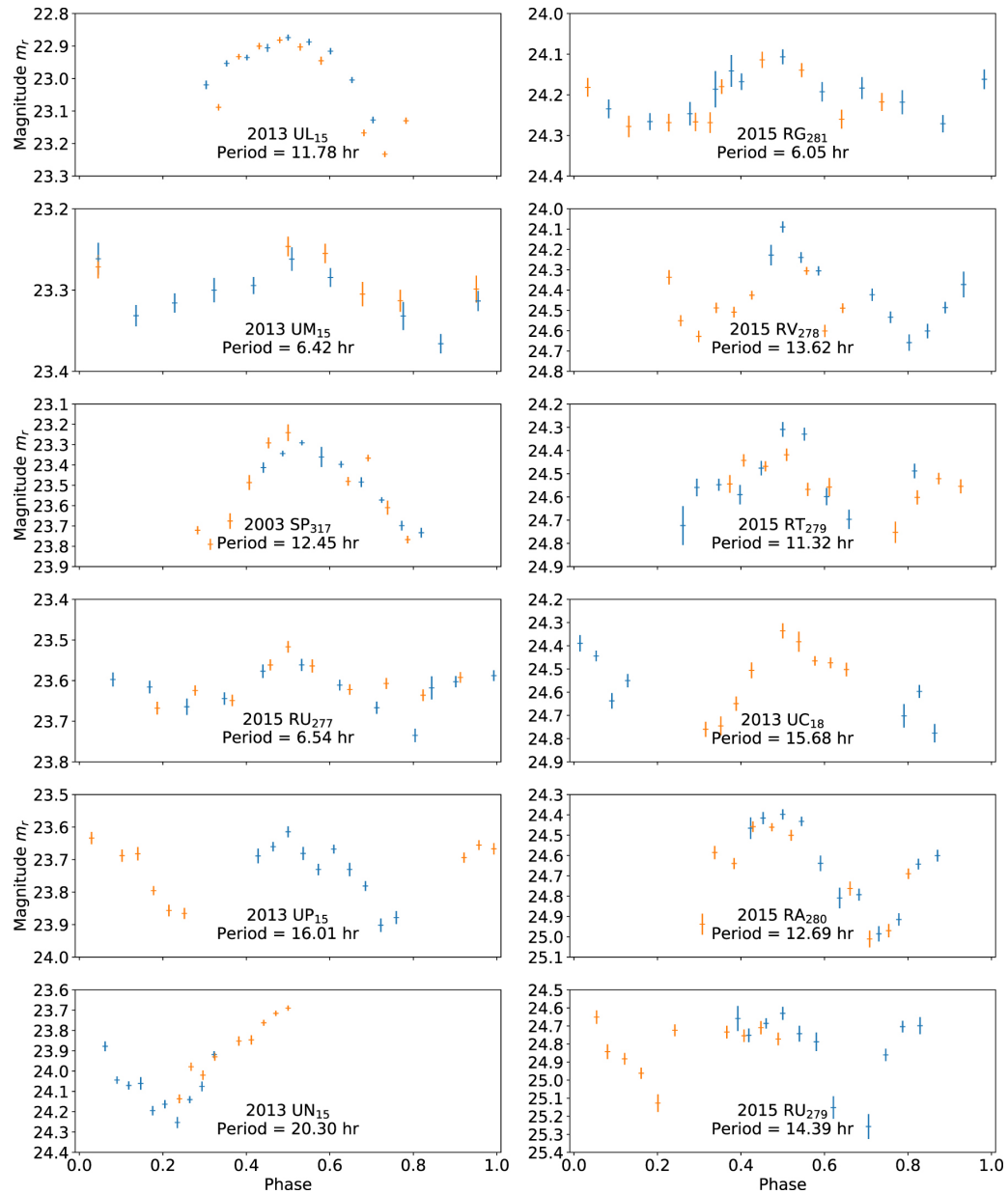
Figure 8. from OSSOS. XII. Variability Studies of 65 Trans-Neptunian Objects Using the Hyper Suprime-Cam null 2019 APJS 244 19 doi:10.3847/1538-4365/ab2fe4 https://dx.doi.org/10.3847/1538-4365/ab2fe4
