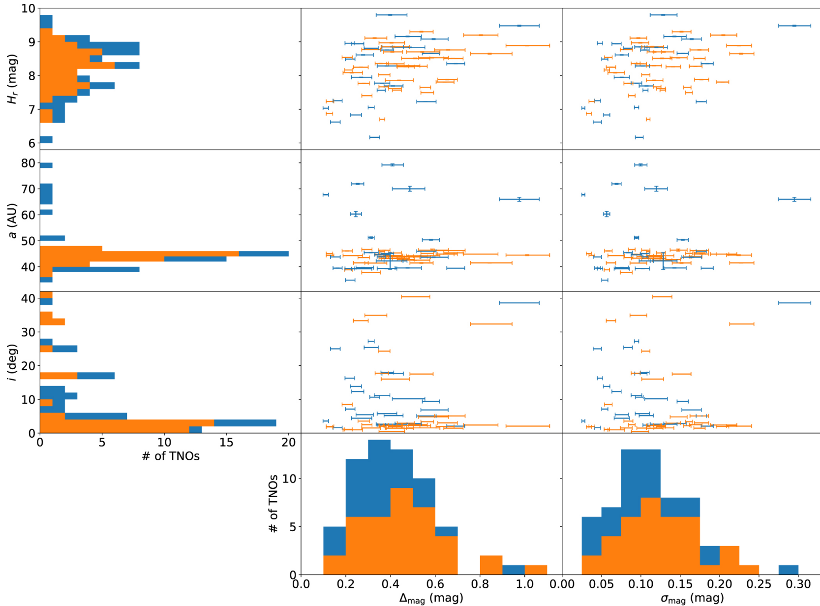
Figure 7. from OSSOS. XII. Variability Studies of 65 Trans-Neptunian Objects Using the Hyper Suprime-Cam null 2019 APJS 244 19 doi:10.3847/1538-4365/ab2fe4 https://dx.doi.org/10.3847/1538-4365/ab2fe4 © 2019. The American Astronomical Society. All rights reserved.
