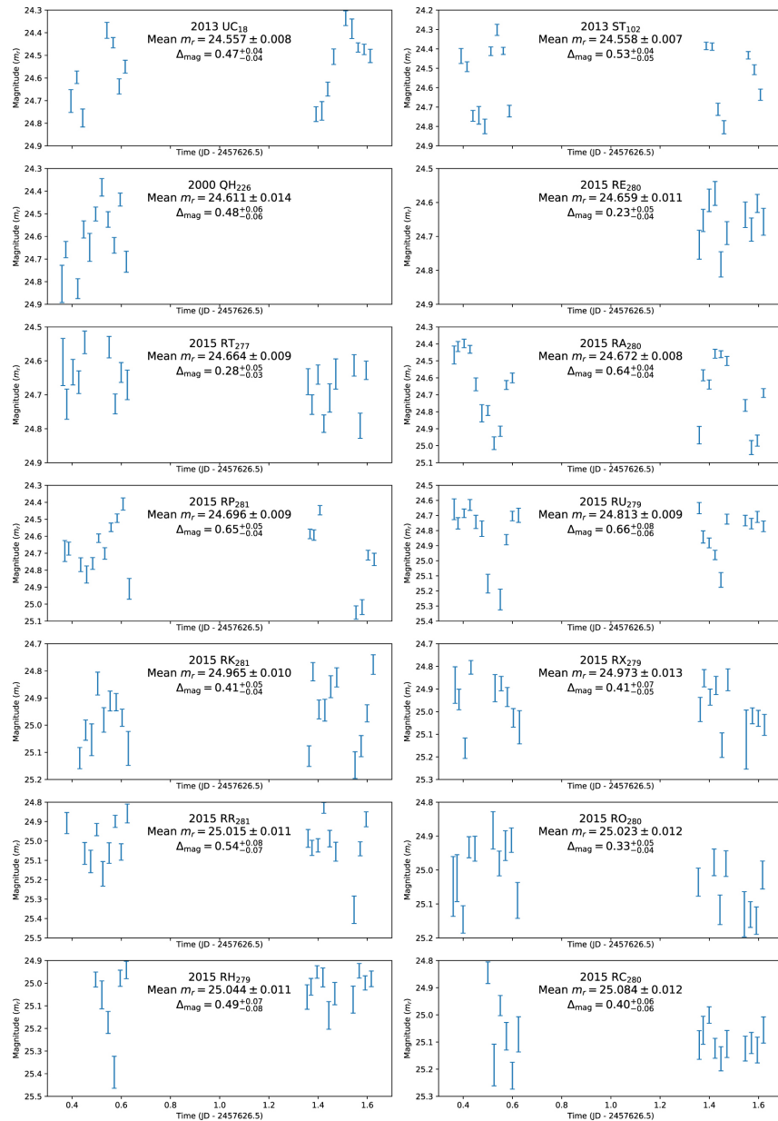
Figure 5. from OSSOS. XII. Variability Studies of 65 Trans-Neptunian Objects Using the Hyper Suprime-Cam null 2019 APJS 244 19 doi:10.3847/1538-4365/ab2fe4 https://dx.doi.org/10.3847/1538-4365/ab2fe4
