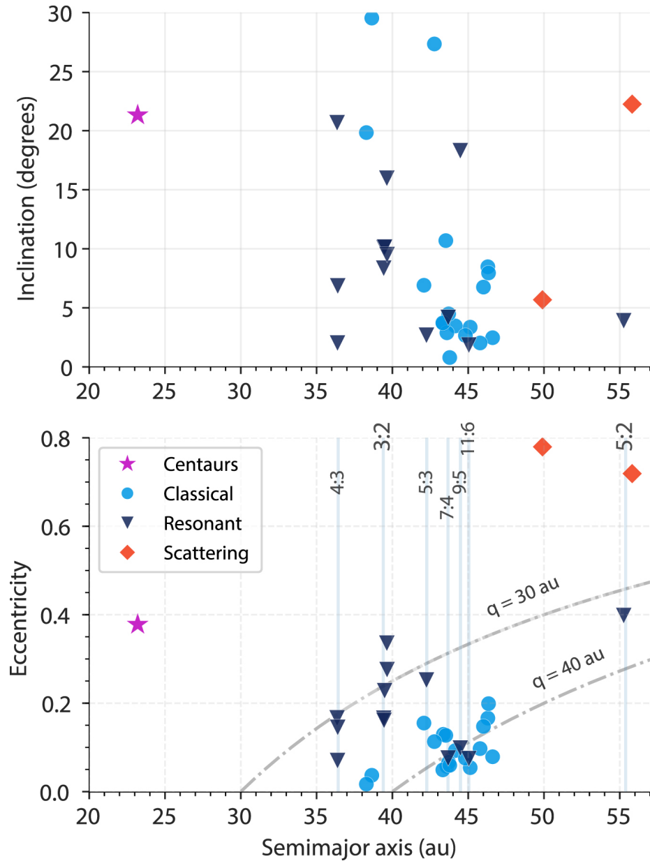
Figure 3. from Col-OSSOS: The Colors of the Outer Solar System Origins Survey null 2019 APJS 243 12 doi:10.3847/1538-4365/ab2194 https://dx.doi.org/10.3847/1538-4365/ab2194
