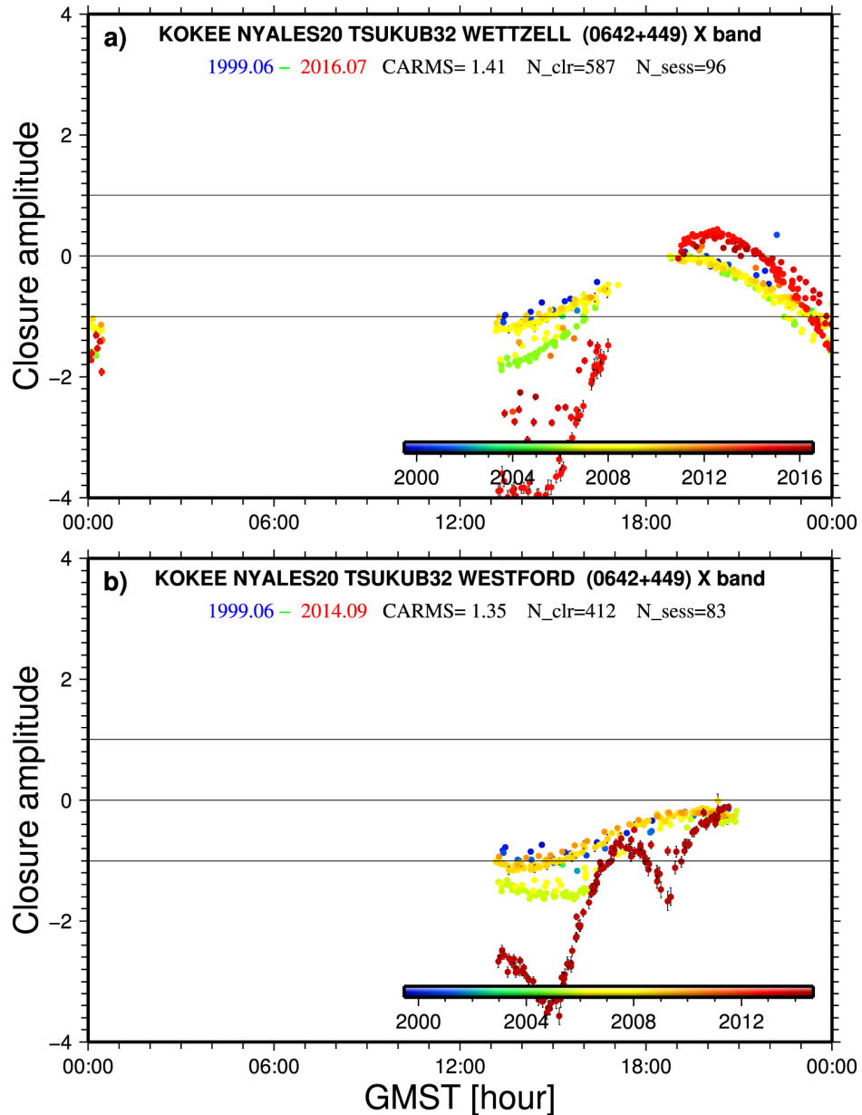
Figure 8. from Structure Effects for 3417 Celestial Reference Frame Radio Sources null 2019 APJS 242 5 doi:10.3847/1538-4365/ab16ea https://dx.doi.org/10.3847/1538-4365/ab16ea © 2019. The American Astronomical Society.
