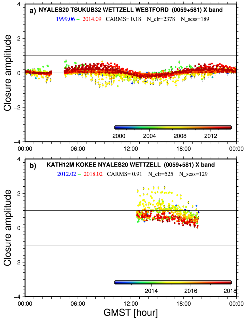
Figure 7. from Structure Effects for 3417 Celestial Reference Frame Radio Sources null 2019 APJS 242 5 doi:10.3847/1538-4365/ab16ea https://dx.doi.org/10.3847/1538-4365/ab16ea © 2019. The American Astronomical Society.
