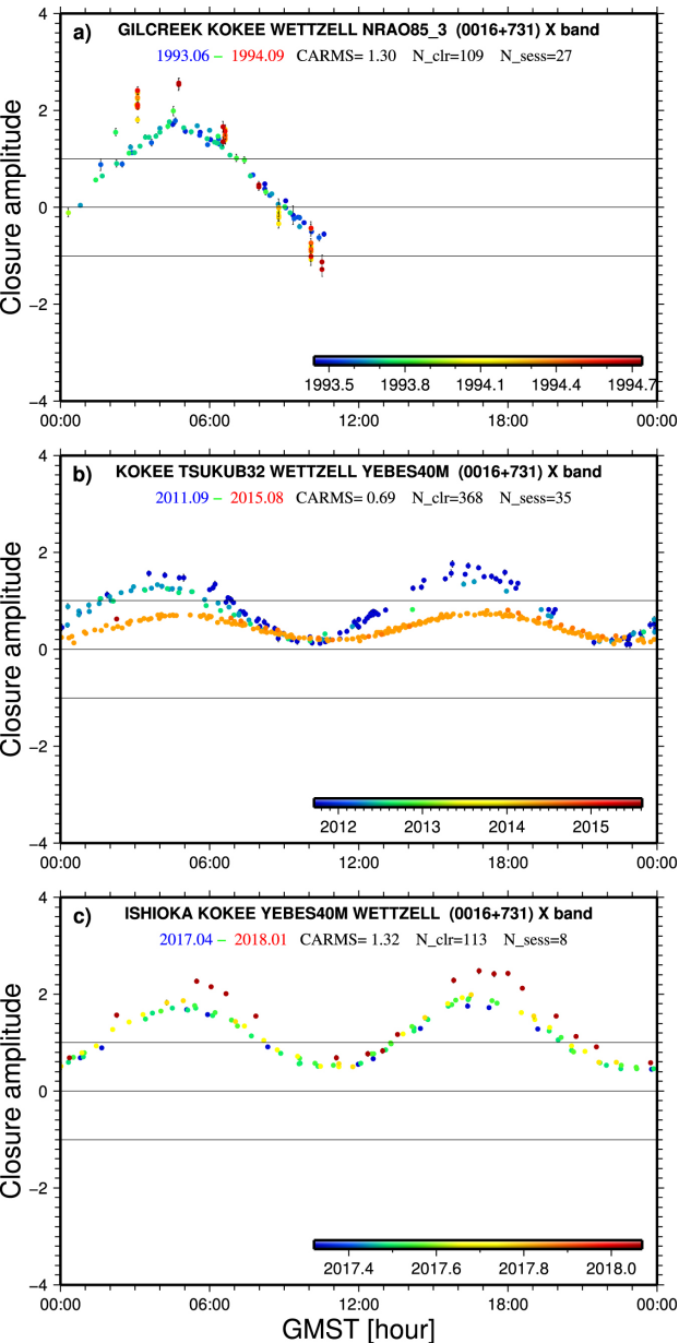
Figure 6. from Structure Effects for 3417 Celestial Reference Frame Radio Sources null 2019 APJS 242 5 doi:10.3847/1538-4365/ab16ea https://dx.doi.org/10.3847/1538-4365/ab16ea © 2019. The American Astronomical Society.
