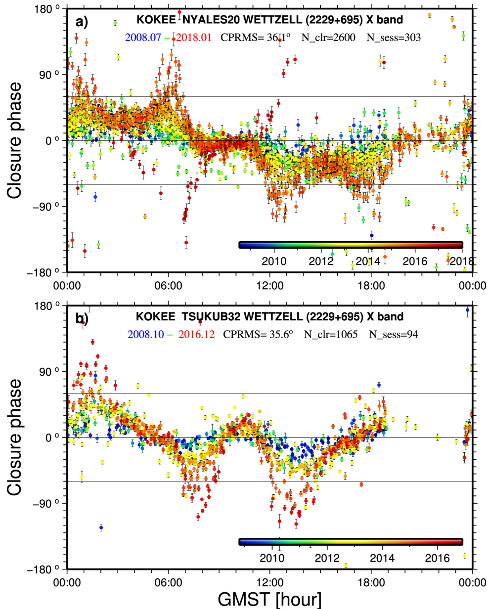
Figure 4. from Structure Effects for 3417 Celestial Reference Frame Radio Sources null 2019 APJS 242 5 doi:10.3847/1538-4365/ab16ea https://dx.doi.org/10.3847/1538-4365/ab16ea © 2019. The American Astronomical Society.
