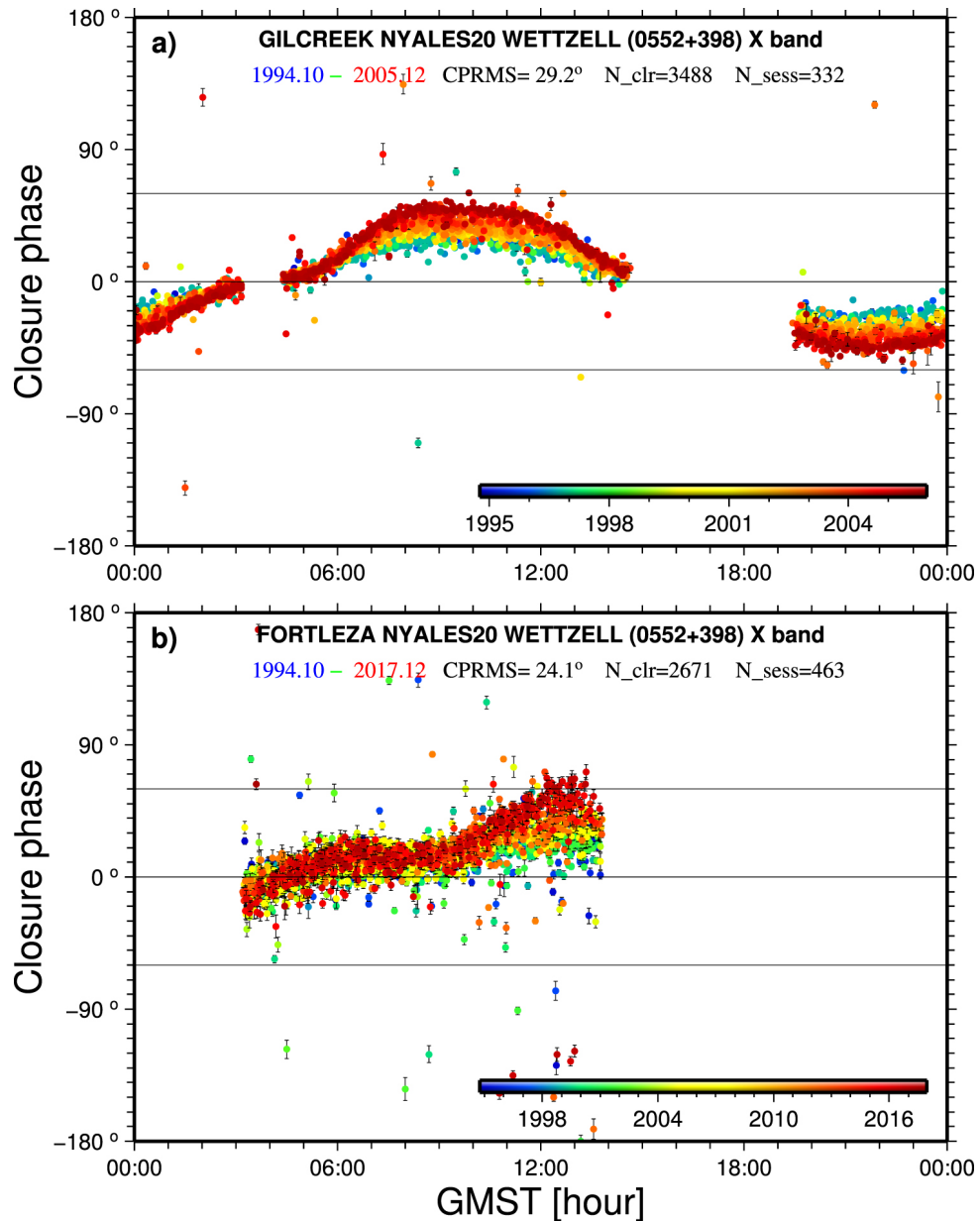
Figure 3. from Structure Effects for 3417 Celestial Reference Frame Radio Sources null 2019 APJS 242 5 doi:10.3847/1538-4365/ab16ea https://dx.doi.org/10.3847/1538-4365/ab16ea © 2019. The American Astronomical Society.
