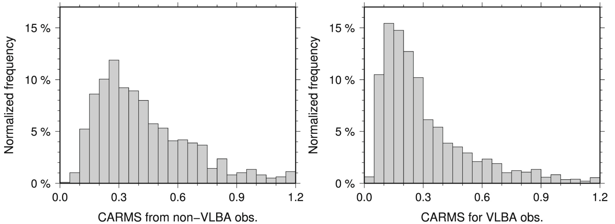
Figure 19. from Structure Effects for 3417 Celestial Reference Frame Radio Sources null 2019 APJS 242 5 doi:10.3847/1538-4365/ab16ea https://dx.doi.org/10.3847/1538-4365/ab16ea © 2019. The American Astronomical Society.
