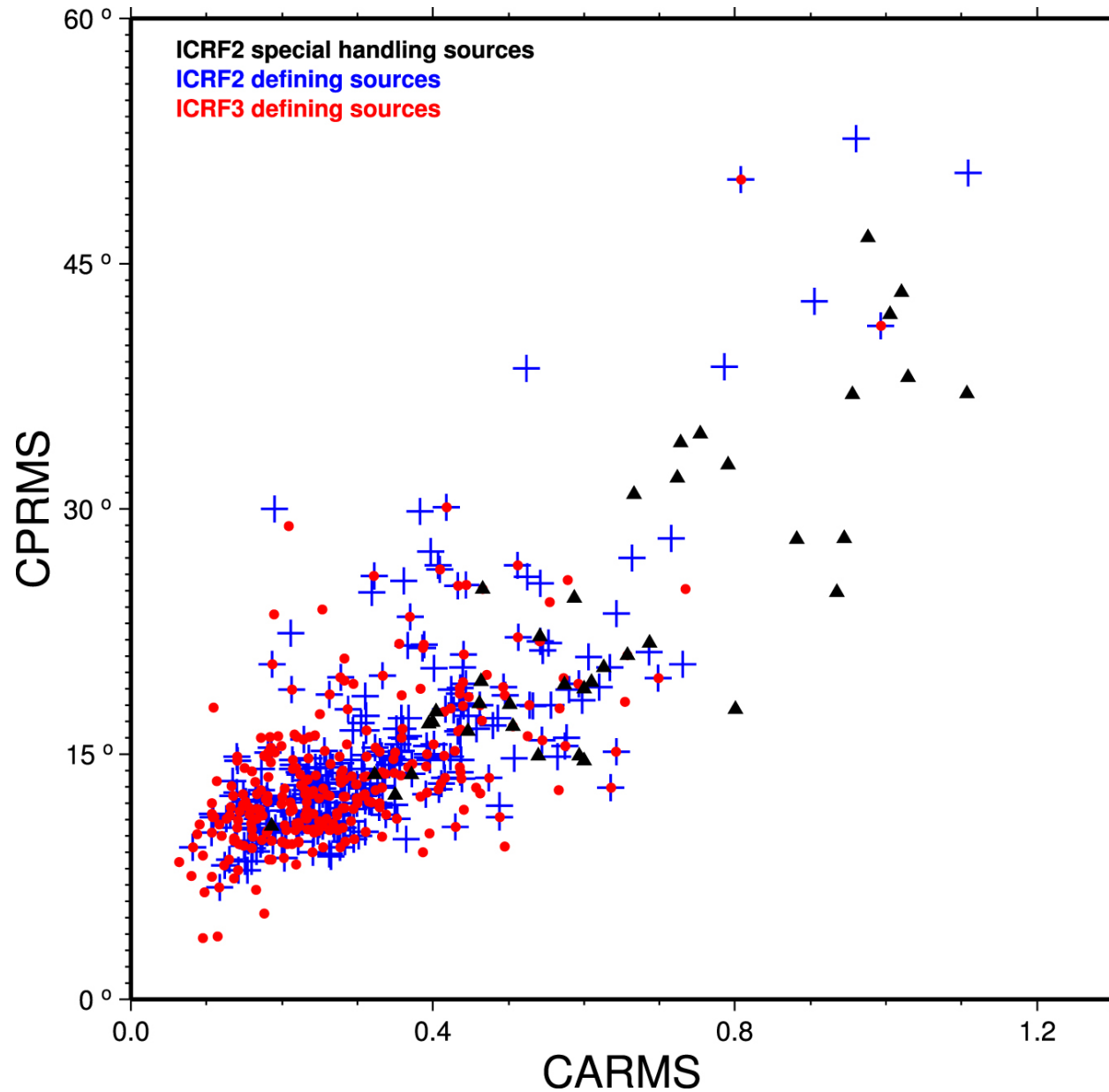
Figure 18. from Structure Effects for 3417 Celestial Reference Frame Radio Sources null 2019 APJS 242 5 doi:10.3847/1538-4365/ab16ea https://dx.doi.org/10.3847/1538-4365/ab16ea © 2019. The American Astronomical Society.
