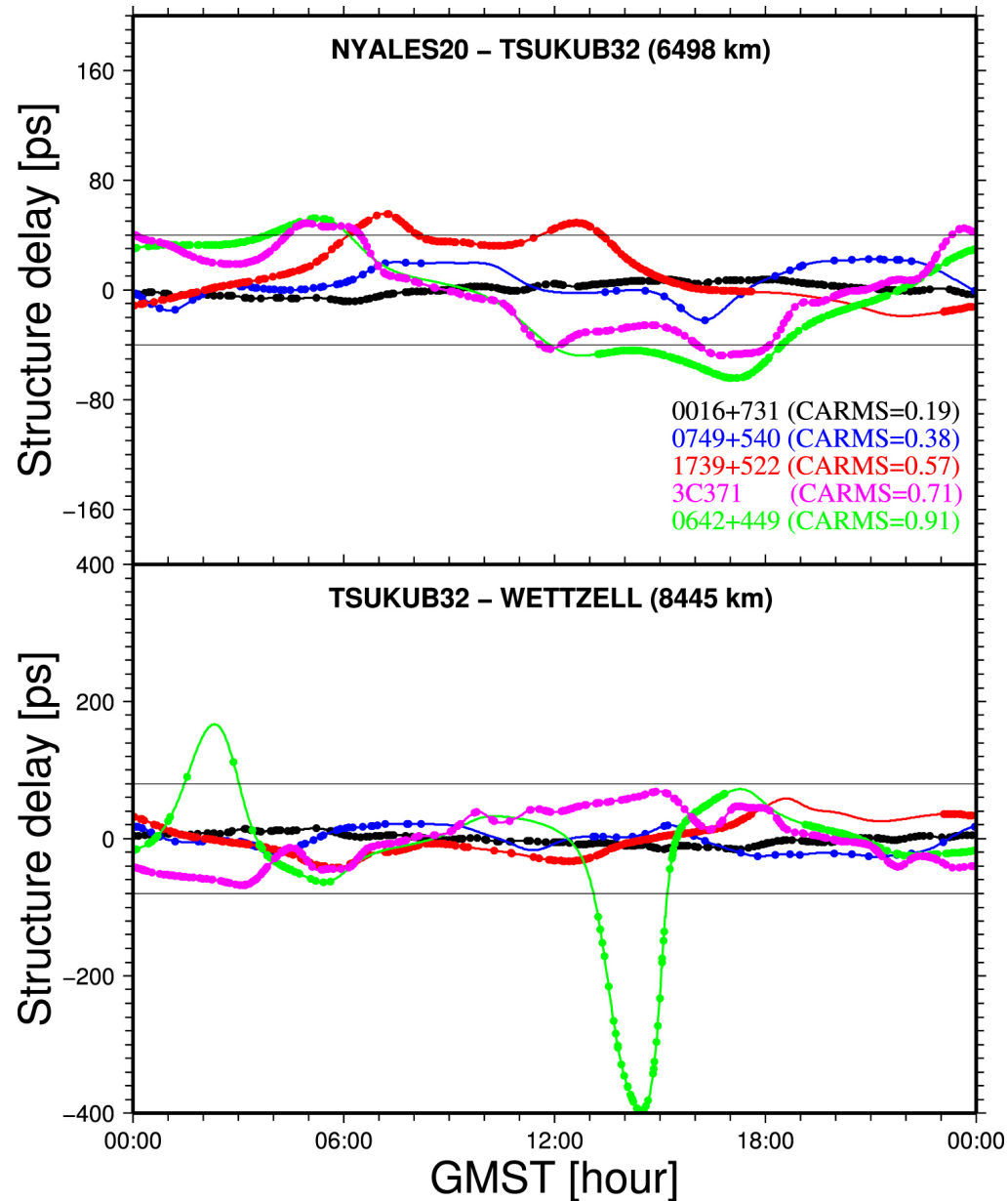
Figure 16. from Structure Effects for 3417 Celestial Reference Frame Radio Sources null 2019 APJS 242 5 doi:10.3847/1538-4365/ab16ea https://dx.doi.org/10.3847/1538-4365/ab16ea © 2019. The American Astronomical Society.
