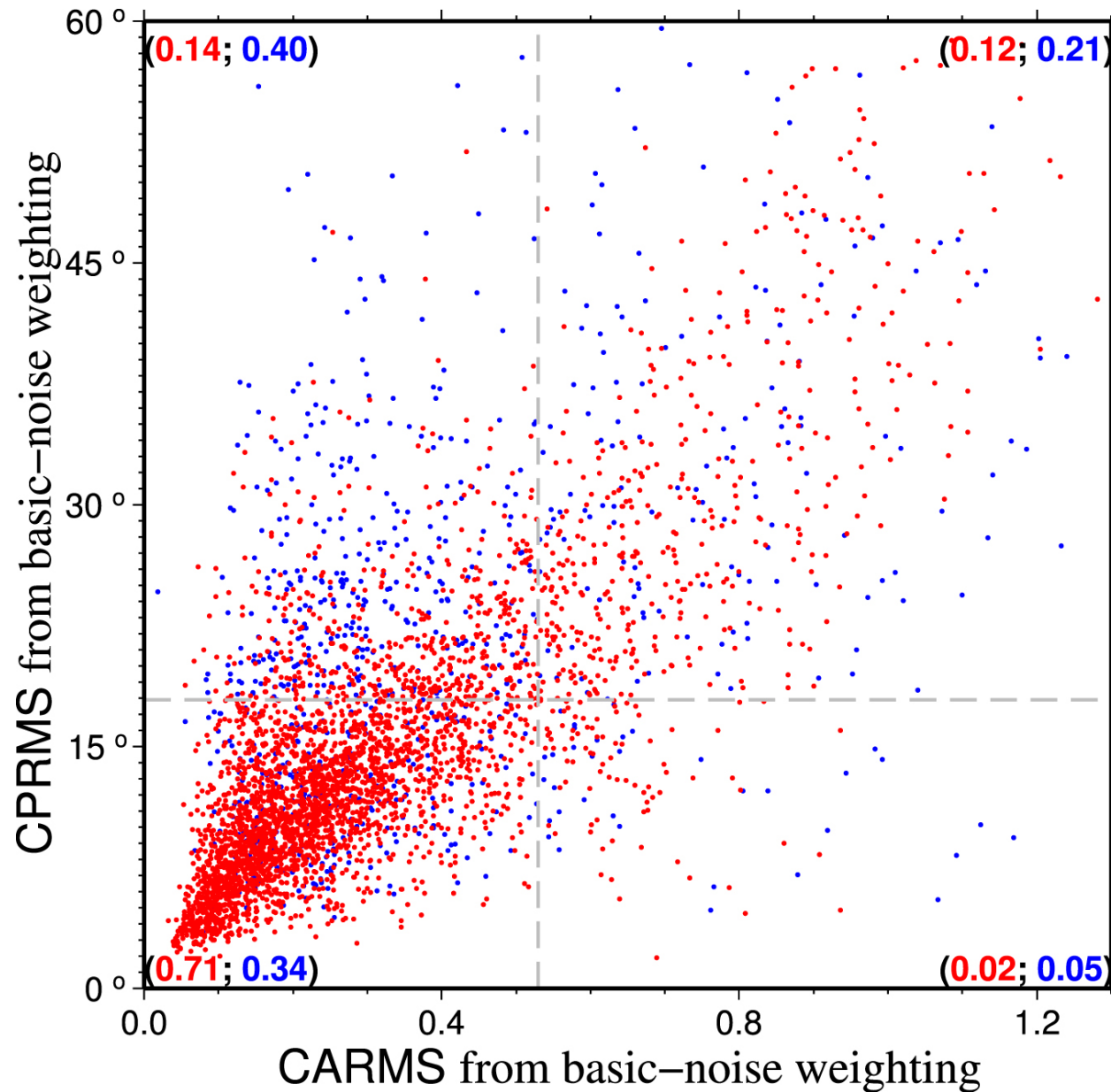
Figure 15. from Structure Effects for 3417 Celestial Reference Frame Radio Sources null 2019 APJS 242 5 doi:10.3847/1538-4365/ab16ea https://dx.doi.org/10.3847/1538-4365/ab16ea © 2019. The American Astronomical Society.
