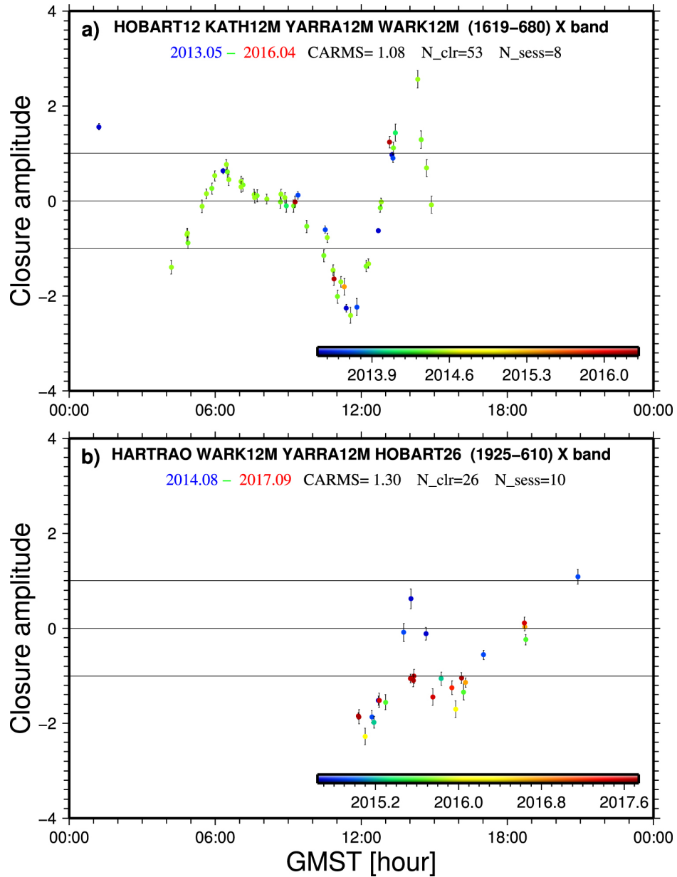
Figure 13. from Structure Effects for 3417 Celestial Reference Frame Radio Sources null 2019 APJS 242 5 doi:10.3847/1538-4365/ab16ea https://dx.doi.org/10.3847/1538-4365/ab16ea © 2019. The American Astronomical Society.
