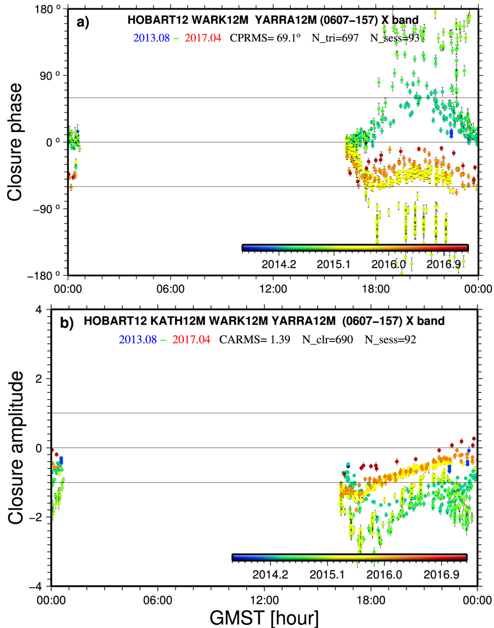
Figure 12. from Structure Effects for 3417 Celestial Reference Frame Radio Sources null 2019 APJS 242 5 doi:10.3847/1538-4365/ab16ea https://dx.doi.org/10.3847/1538-4365/ab16ea © 2019. The American Astronomical Society.
