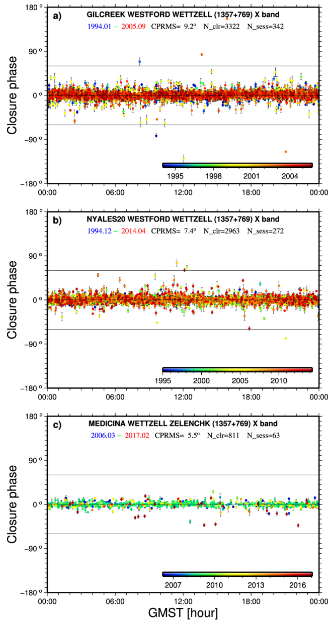
Figure 1. from Structure Effects for 3417 Celestial Reference Frame Radio Sources null 2019 APJS 242 5 doi:10.3847/1538-4365/ab16ea https://dx.doi.org/10.3847/1538-4365/ab16ea © 2019. The American Astronomical Society.
