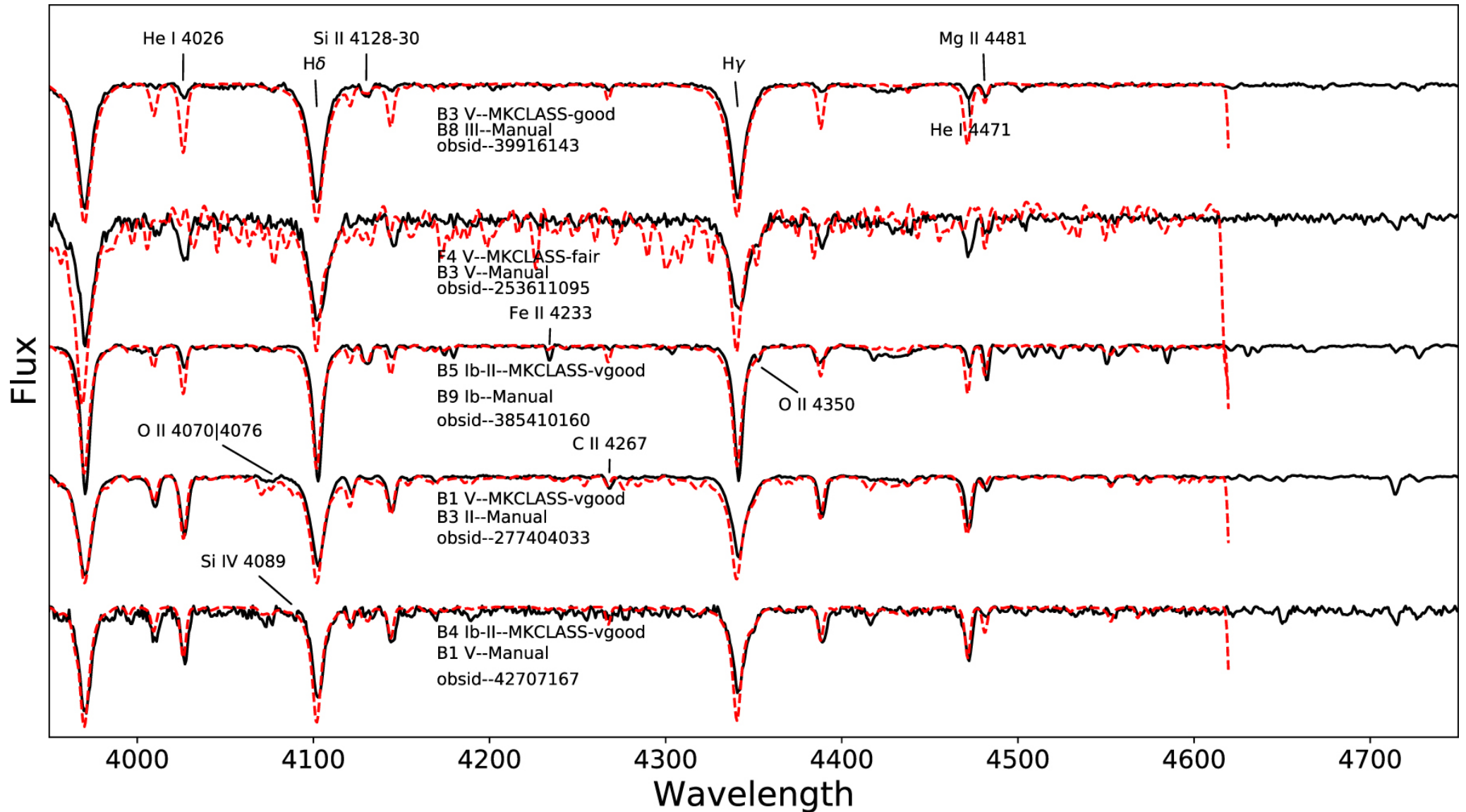
Figure 15. from A Catalog of OB Stars from LAMOST Spectroscopic Survey null 2019 APJS 241 32 doi:10.3847/1538-4365/ab0a0d https://dx.doi.org/10.3847/1538-4365/ab0a0d © 2019. The American Astronomical Society. All rights reserved.
