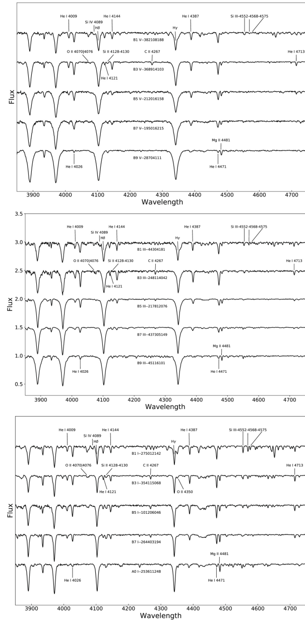
Figure 13. from A Catalog of OB Stars from LAMOST Spectroscopic Survey null 2019 APJS 241 32 doi:10.3847/1538-4365/ab0a0d https://dx.doi.org/10.3847/1538-4365/ab0a0d © 2019. The American Astronomical Society. All rights reserved.
