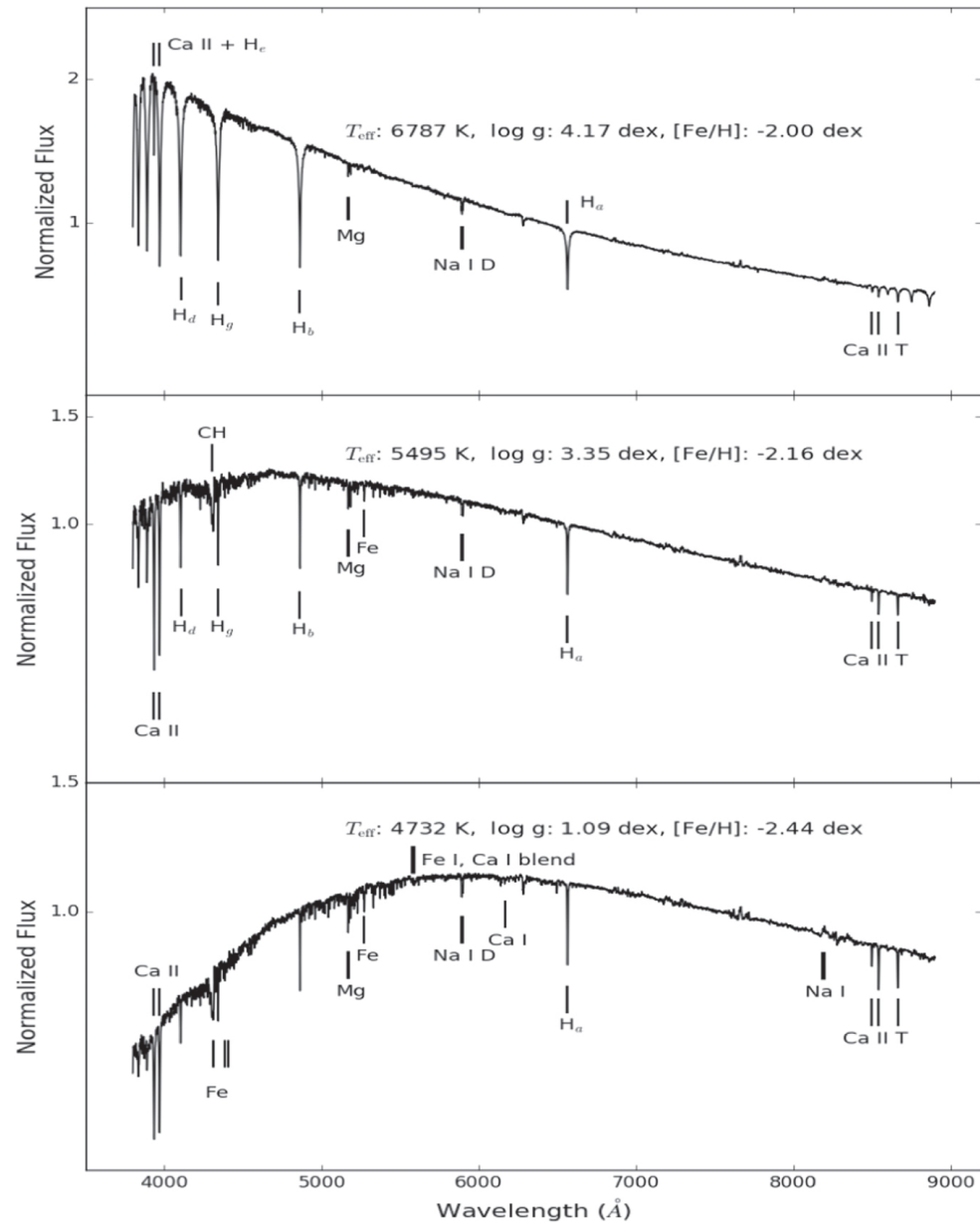
Figure 6. from An Empirical Template Library for FGK and Late-type A Stars Using LAMOST Observed Spectra null 2019 APJS 240 10 doi:10.3847/1538-4365/aaef3c https://dx.doi.org/10.3847/1538-4365/aaef3c © 2019. The American Astronomical Society. All rights reserved.
