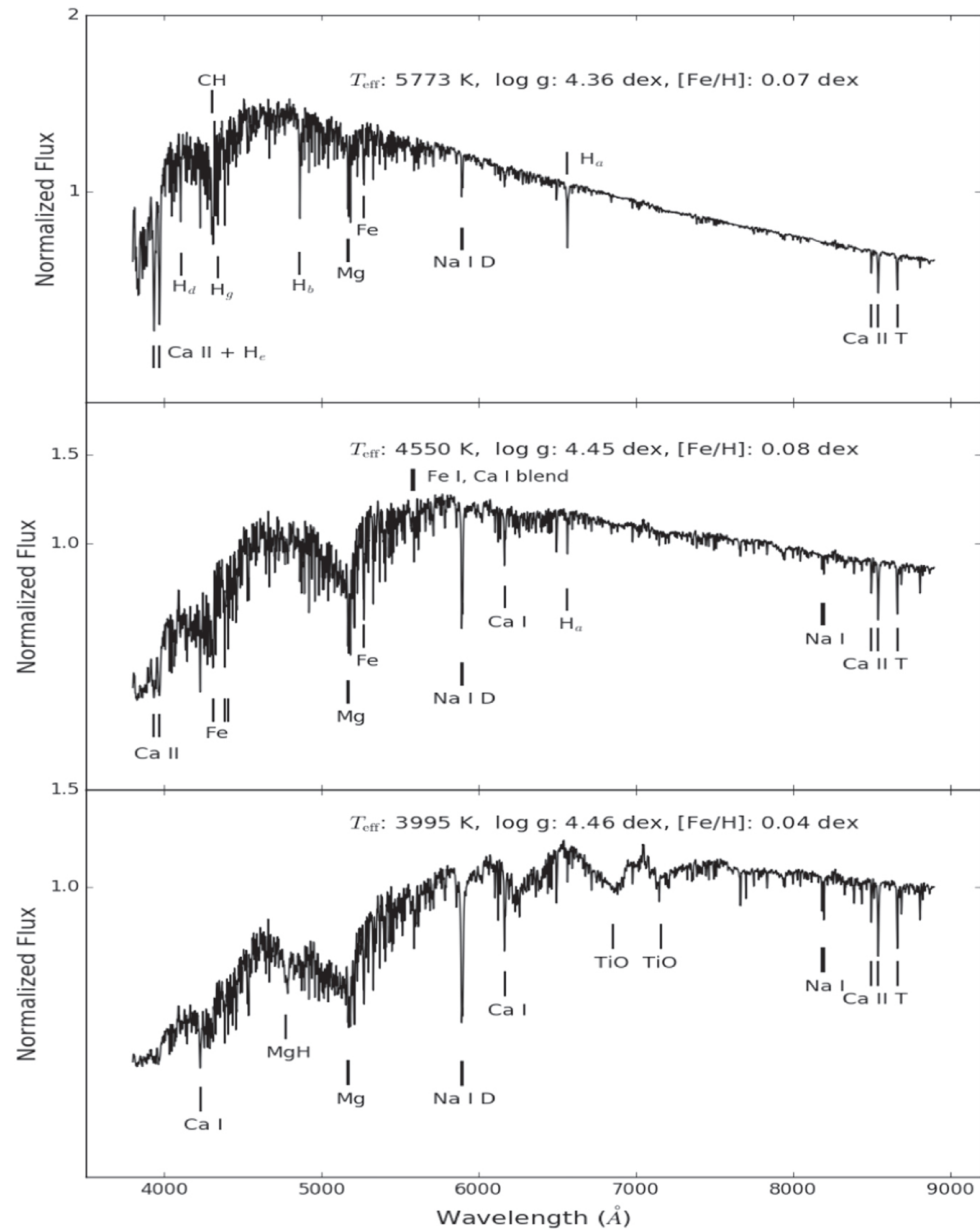
Figure 5. from An Empirical Template Library for FGK and Late-type A Stars Using LAMOST Observed Spectra null 2019 APJS 240 10 doi:10.3847/1538-4365/aaef3c https://dx.doi.org/10.3847/1538-4365/aaef3c © 2019. The American Astronomical Society. All rights reserved.
