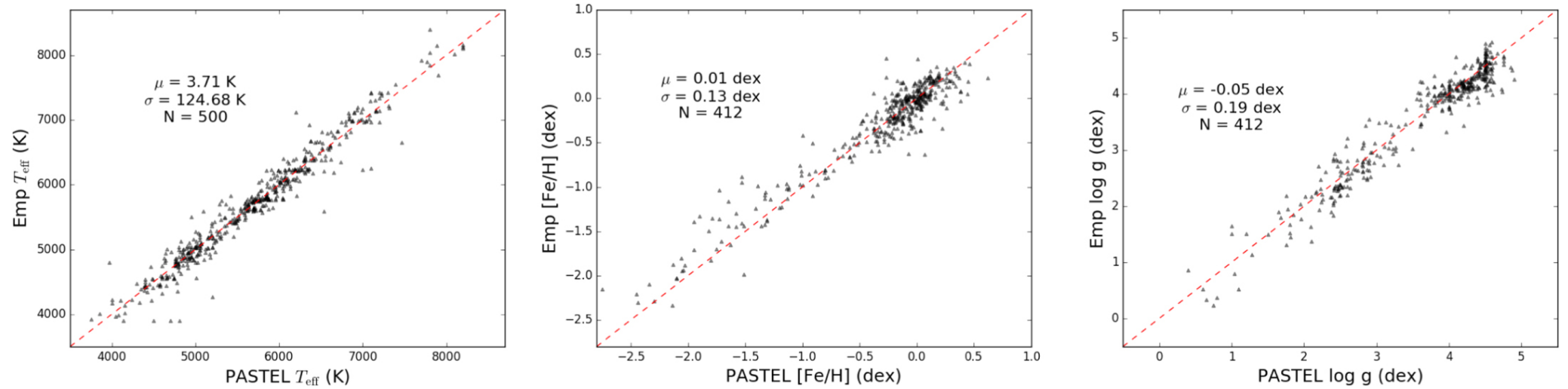
Figure 18. from An Empirical Template Library for FGK and Late-type A Stars Using LAMOST Observed Spectra null 2019 APJS 240 10 doi:10.3847/1538-4365/aaef3c https://dx.doi.org/10.3847/1538-4365/aaef3c © 2019. The American Astronomical Society. All rights reserved.
