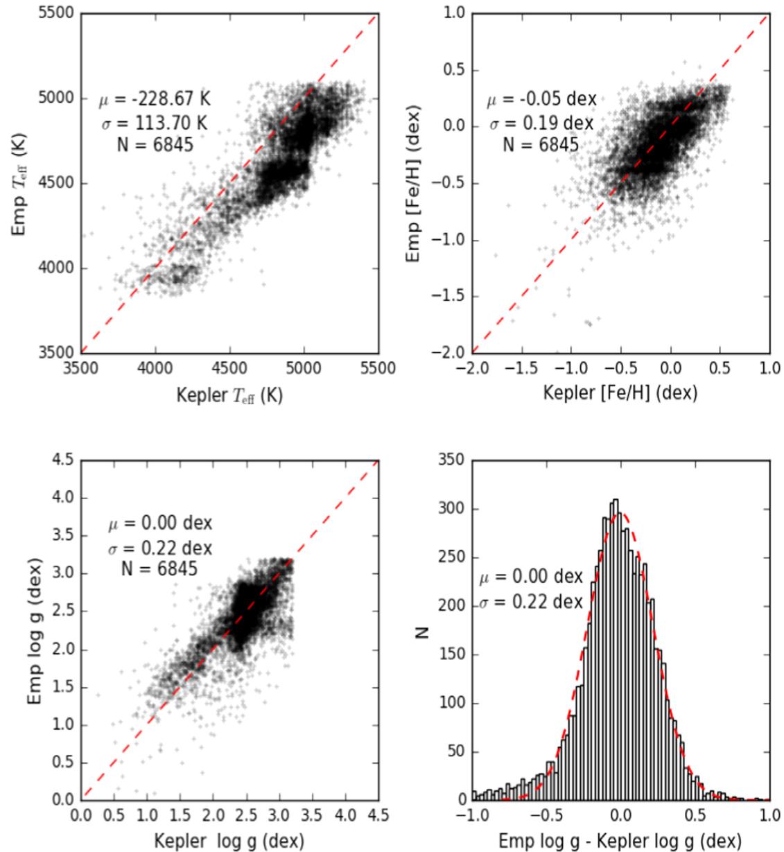
Figure 16. from An Empirical Template Library for FGK and Late-type A Stars Using LAMOST Observed Spectra null 2019 APJS 240 10 doi:10.3847/1538-4365/aaef3c https://dx.doi.org/10.3847/1538-4365/aaef3c
