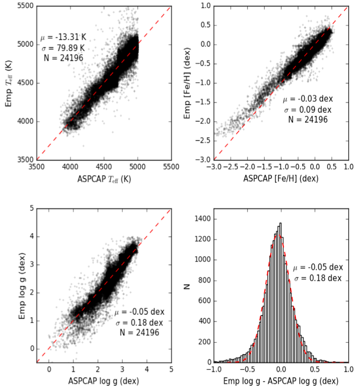
Figure 15. from An Empirical Template Library for FGK and Late-type A Stars Using LAMOST Observed Spectra null 2019 APJS 240 10 doi:10.3847/1538-4365/aaef3c https://dx.doi.org/10.3847/1538-4365/aaef3c
