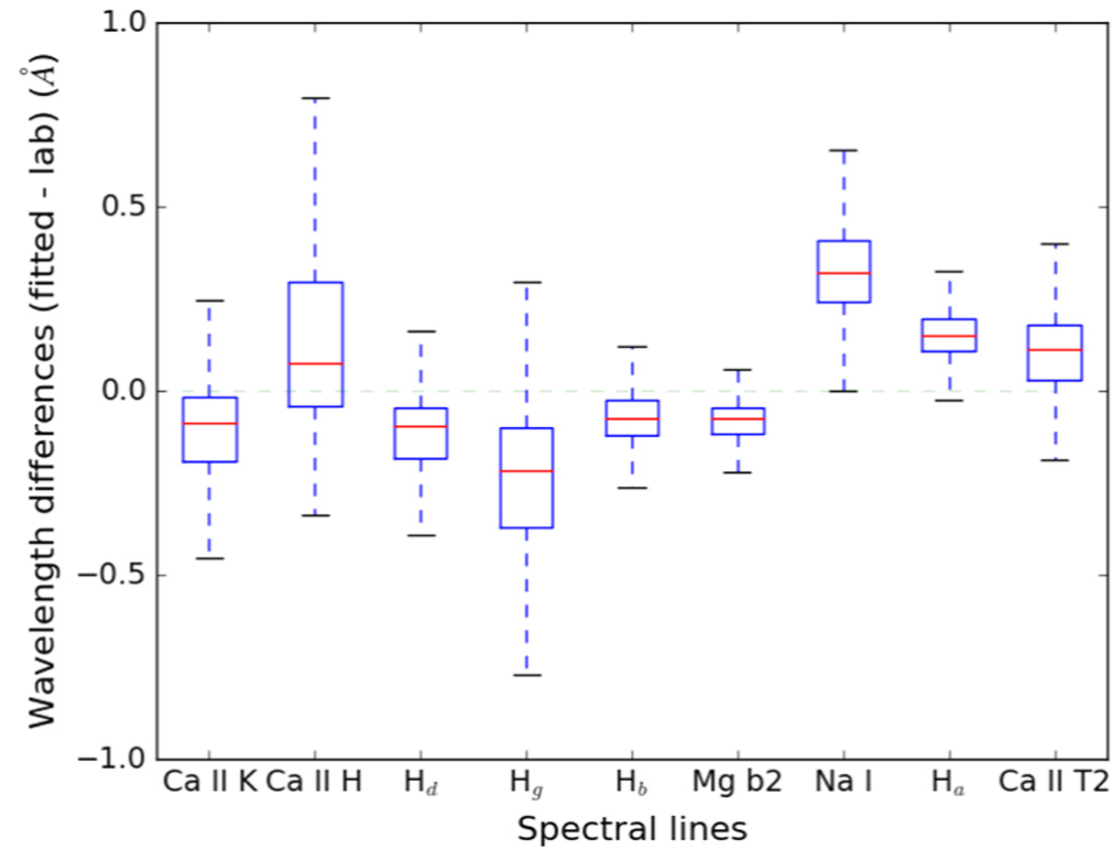
Figure 13. from An Empirical Template Library for FGK and Late-type A Stars Using LAMOST Observed Spectra null 2019 APJS 240 10 doi:10.3847/1538-4365/aaef3c https://dx.doi.org/10.3847/1538-4365/aaef3c © 2019. The American Astronomical Society. All rights reserved.
