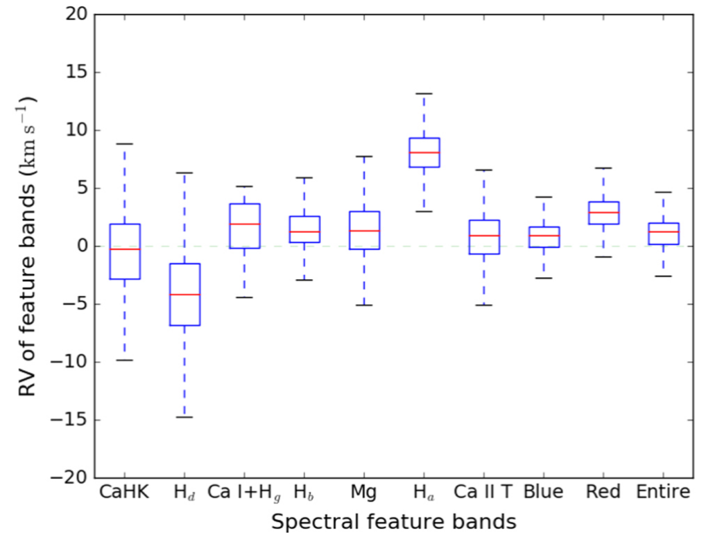
Figure 13. from An Empirical Template Library for FGK and Late-type A Stars Using LAMOST Observed Spectra null 2019 APJS 240 10 doi:10.3847/1538-4365/aaef3c https://dx.doi.org/10.3847/1538-4365/aaef3c © 2019. The American Astronomical Society. All rights reserved.
