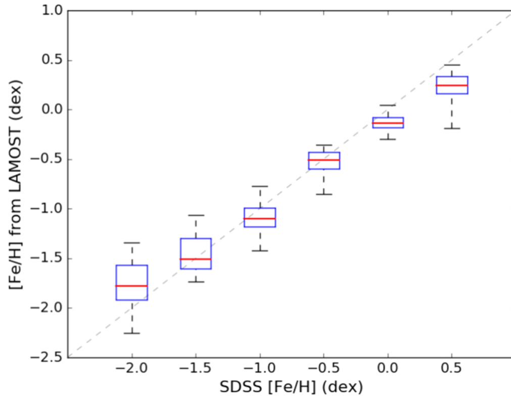
Figure 10. from An Empirical Template Library for FGK and Late-type A Stars Using LAMOST Observed Spectra null 2019 APJS 240 10 doi:10.3847/1538-4365/aaef3c https://dx.doi.org/10.3847/1538-4365/aaef3c © 2019. The American Astronomical Society. All rights reserved.
