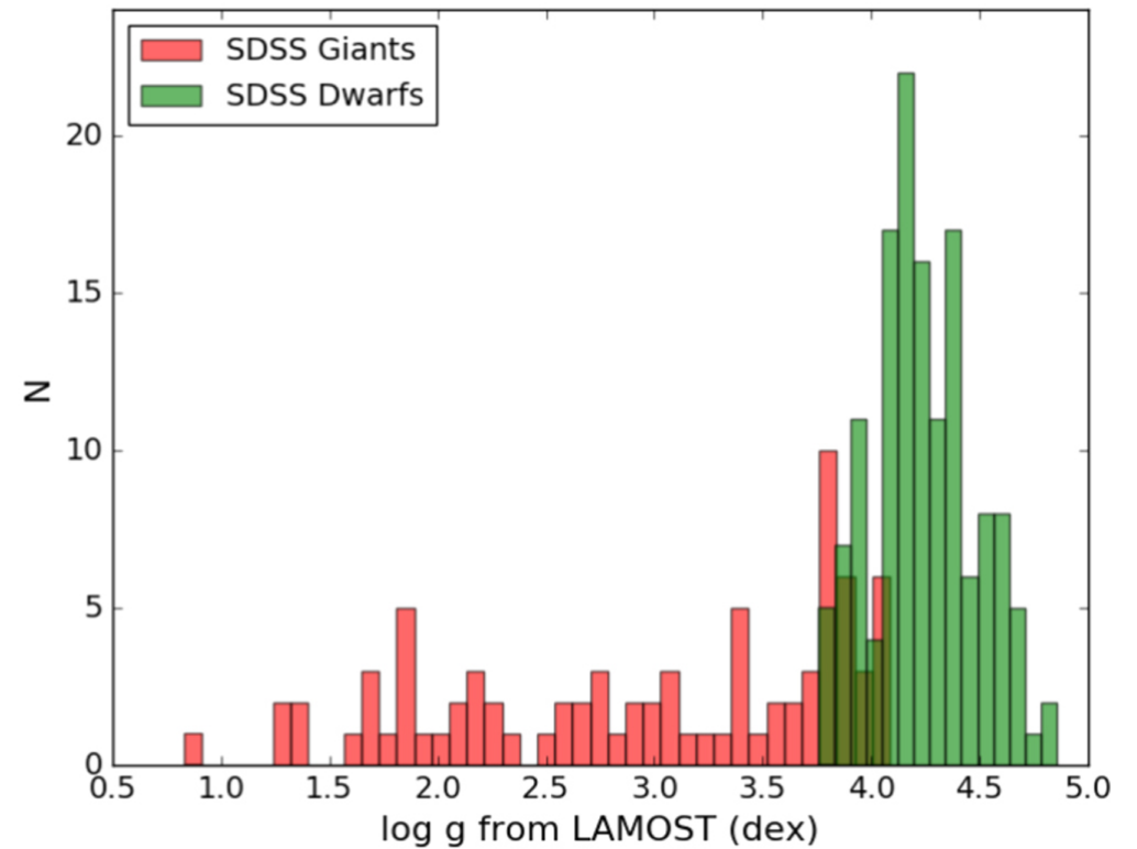
Figure 10. from An Empirical Template Library for FGK and Late-type A Stars Using LAMOST Observed Spectra null 2019 APJS 240 10 doi:10.3847/1538-4365/aaef3c https://dx.doi.org/10.3847/1538-4365/aaef3c © 2019. The American Astronomical Society. All rights reserved.
