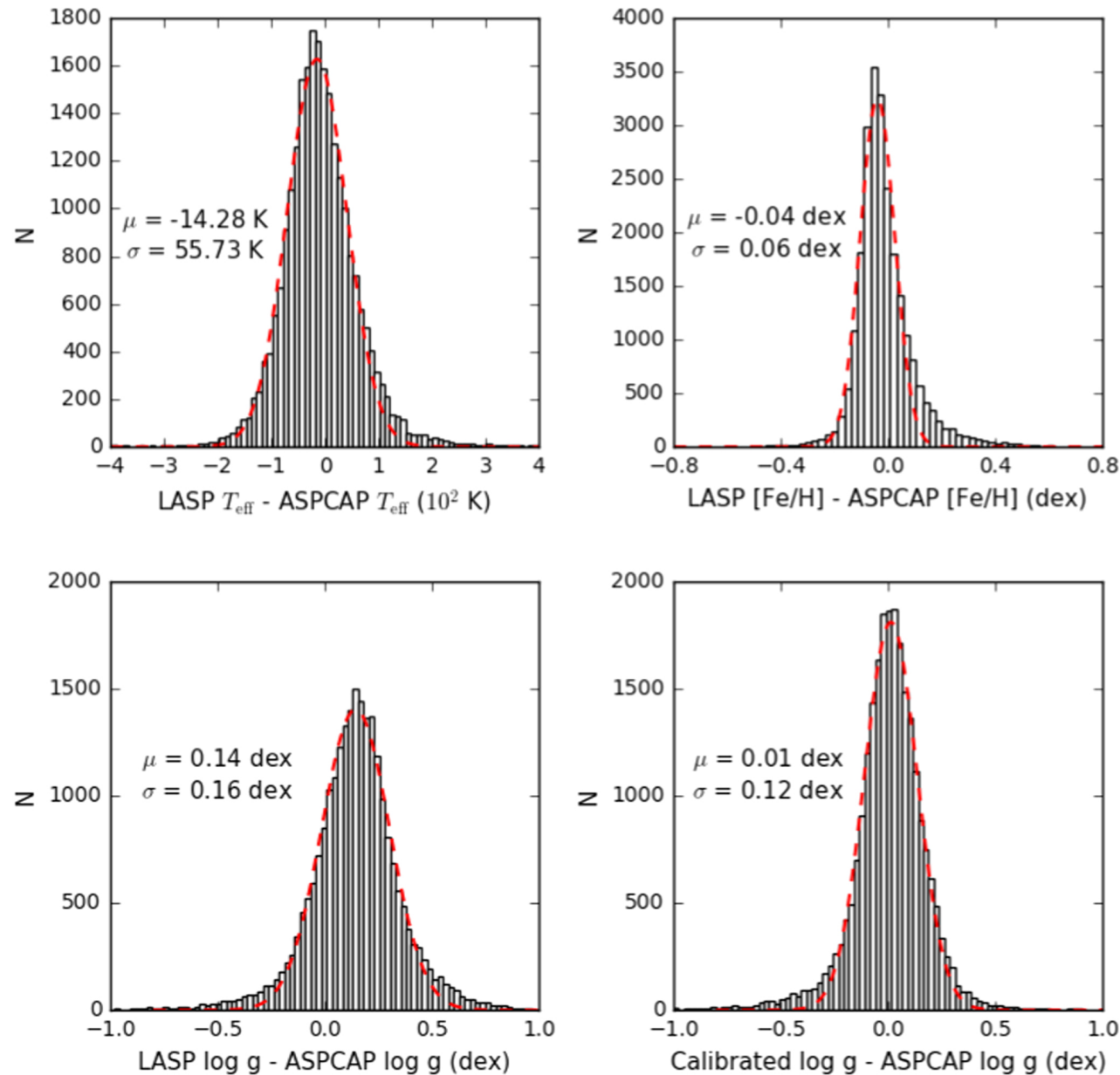
Figure 1. from An Empirical Template Library for FGK and Late-type A Stars Using LAMOST Observed Spectra null 2019 APJS 240 10 doi:10.3847/1538-4365/aaef3c https://dx.doi.org/10.3847/1538-4365/aaef3c
