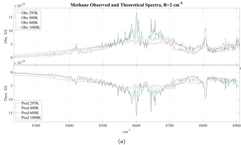
Figure 7. from Atlas of Experimental and Theoretical High-temperature Methane Cross Sections from T = 295 to 1000 K in the Near-infrared null 2019 APJS 240 4 doi:10.3847/1538-4365/aaed39 https://dx.doi.org/10.3847/1538-4365/aaed39 © 2019. The American Astronomical Society. All rights reserved.
