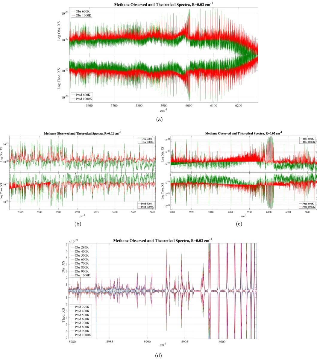
Figure 5. from Atlas of Experimental and Theoretical High-temperature Methane Cross Sections from T = 295 to 1000 K in the Near-infrared null 2019 APJS 240 4 doi:10.3847/1538-4365/aaed39 https://dx.doi.org/10.3847/1538-4365/aaed39 © 2019. The American Astronomical Society. All rights reserved.
