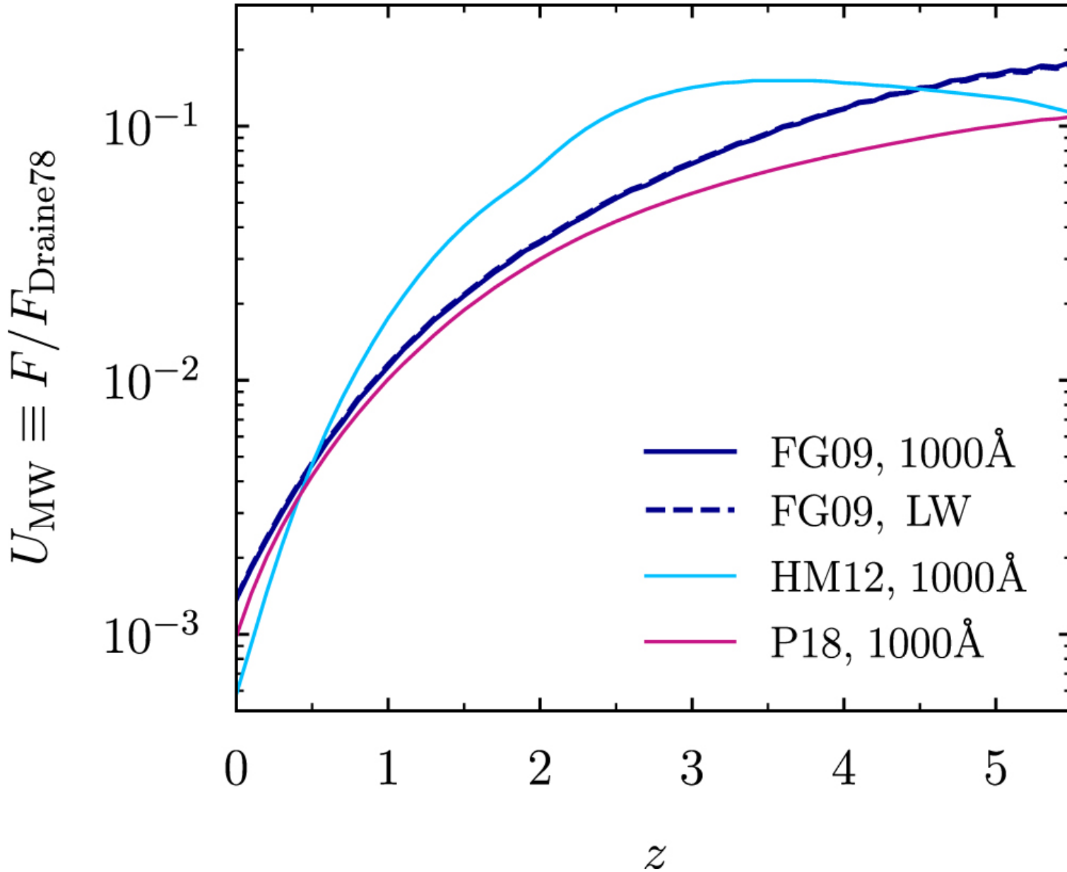
Figure 9. from Modeling the Atomic-to-molecular Transition in Cosmological Simulations of Galaxy Formation null 2018 APJS 238 33 doi:10.3847/1538-4365/aae387 https://dx.doi.org/10.3847/1538-4365/aae387 © 2018. The American Astronomical Society. All rights reserved.
