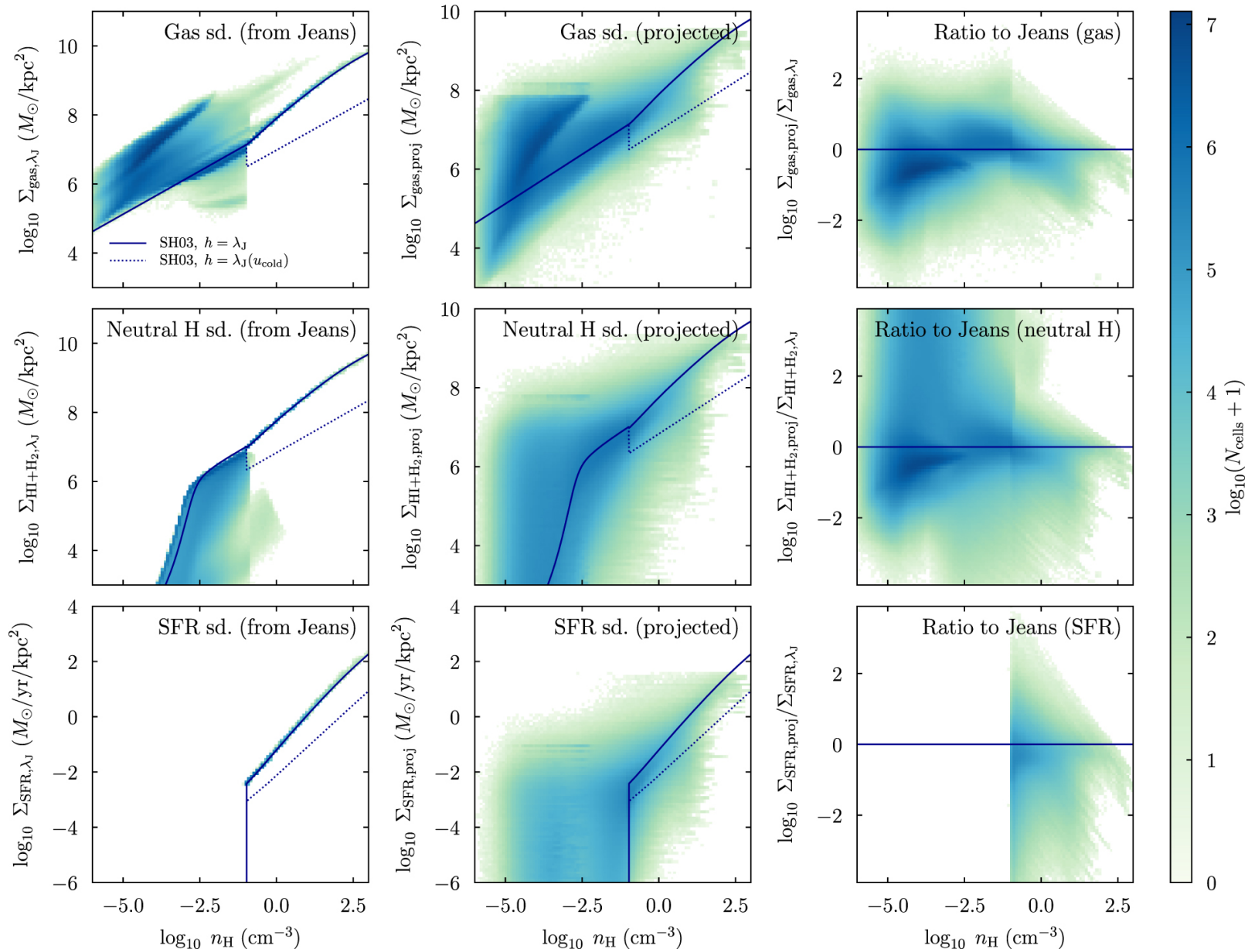
Figure 8. from Modeling the Atomic-to-molecular Transition in Cosmological Simulations of Galaxy Formation null 2018 APJS 238 33 doi:10.3847/1538-4365/aae387 https://dx.doi.org/10.3847/1538-4365/aae387 © 2018. The American Astronomical Society. All rights reserved.
