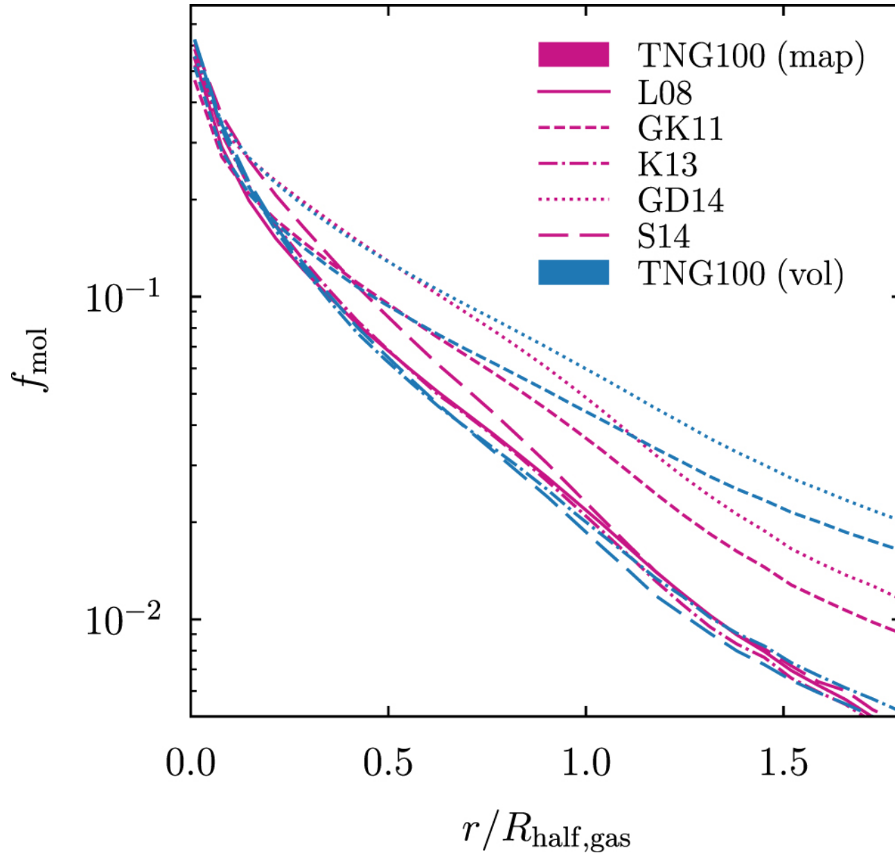
Figure 7. from Modeling the Atomic-to-molecular Transition in Cosmological Simulations of Galaxy Formation null 2018 APJS 238 33 doi:10.3847/1538-4365/aae387 https://dx.doi.org/10.3847/1538-4365/aae387 © 2018. The American Astronomical Society. All rights reserved.
