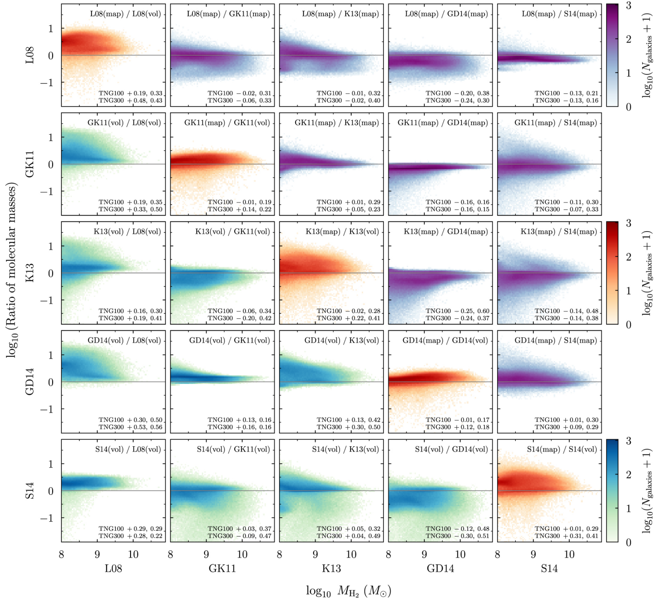
Figure 4. from Modeling the Atomic-to-molecular Transition in Cosmological Simulations of Galaxy Formation null 2018 APJS 238 33 doi:10.3847/1538-4365/aae387 https://dx.doi.org/10.3847/1538-4365/aae387
