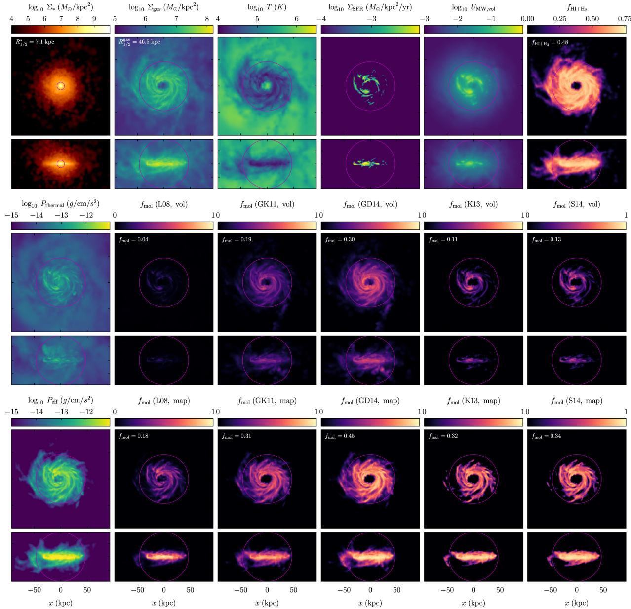
Figure 2. from Modeling the Atomic-to-molecular Transition in Cosmological Simulations of Galaxy Formation null 2018 APJS 238 33 doi:10.3847/1538-4365/aae387 https://dx.doi.org/10.3847/1538-4365/aae387
