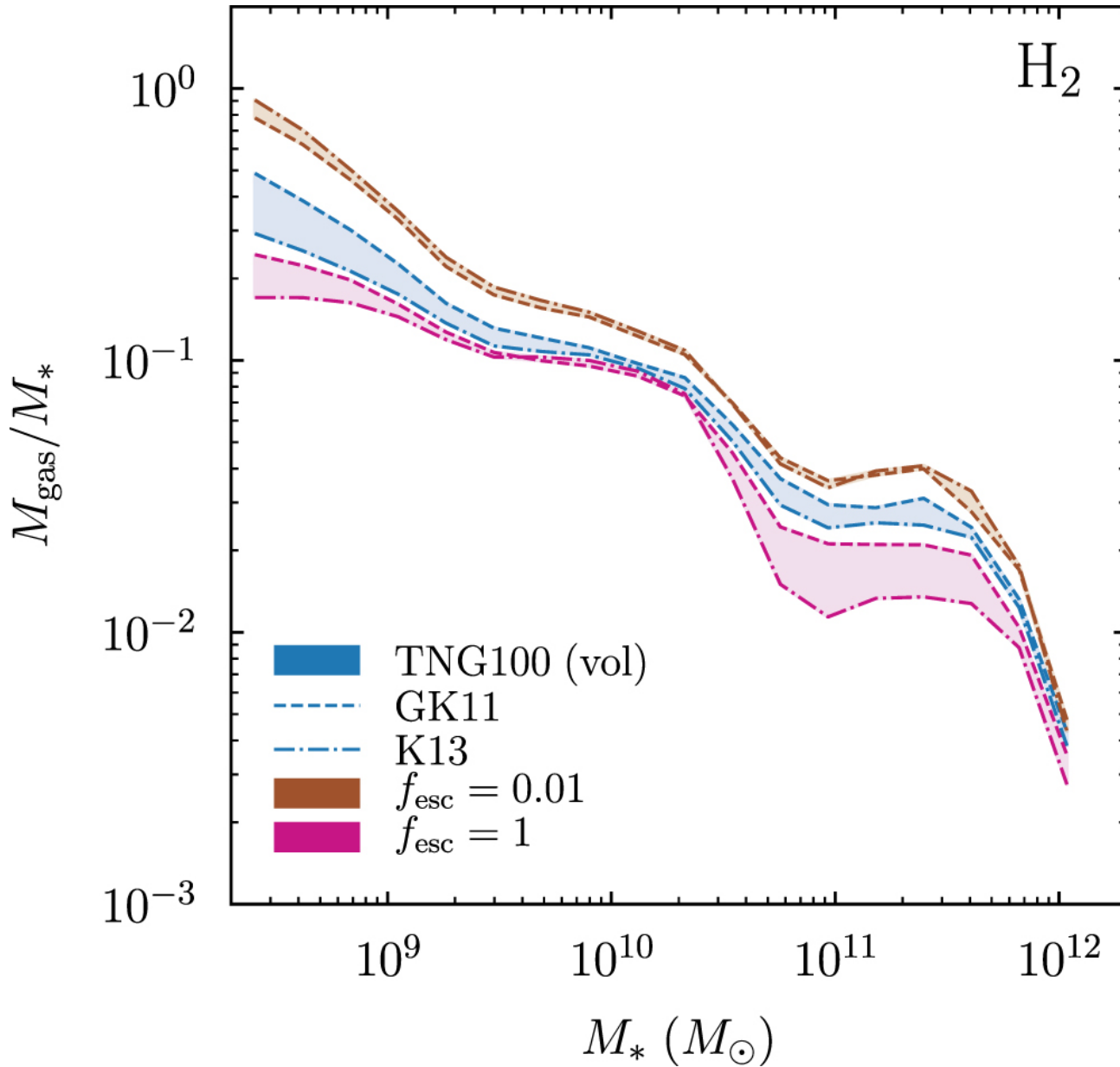
Figure 10. from Modeling the Atomic-to-molecular Transition in Cosmological Simulations of Galaxy Formation null 2018 APJS 238 33 doi:10.3847/1538-4365/aae387 https://dx.doi.org/10.3847/1538-4365/aae387 © 2018. The American Astronomical Society. All rights reserved.
