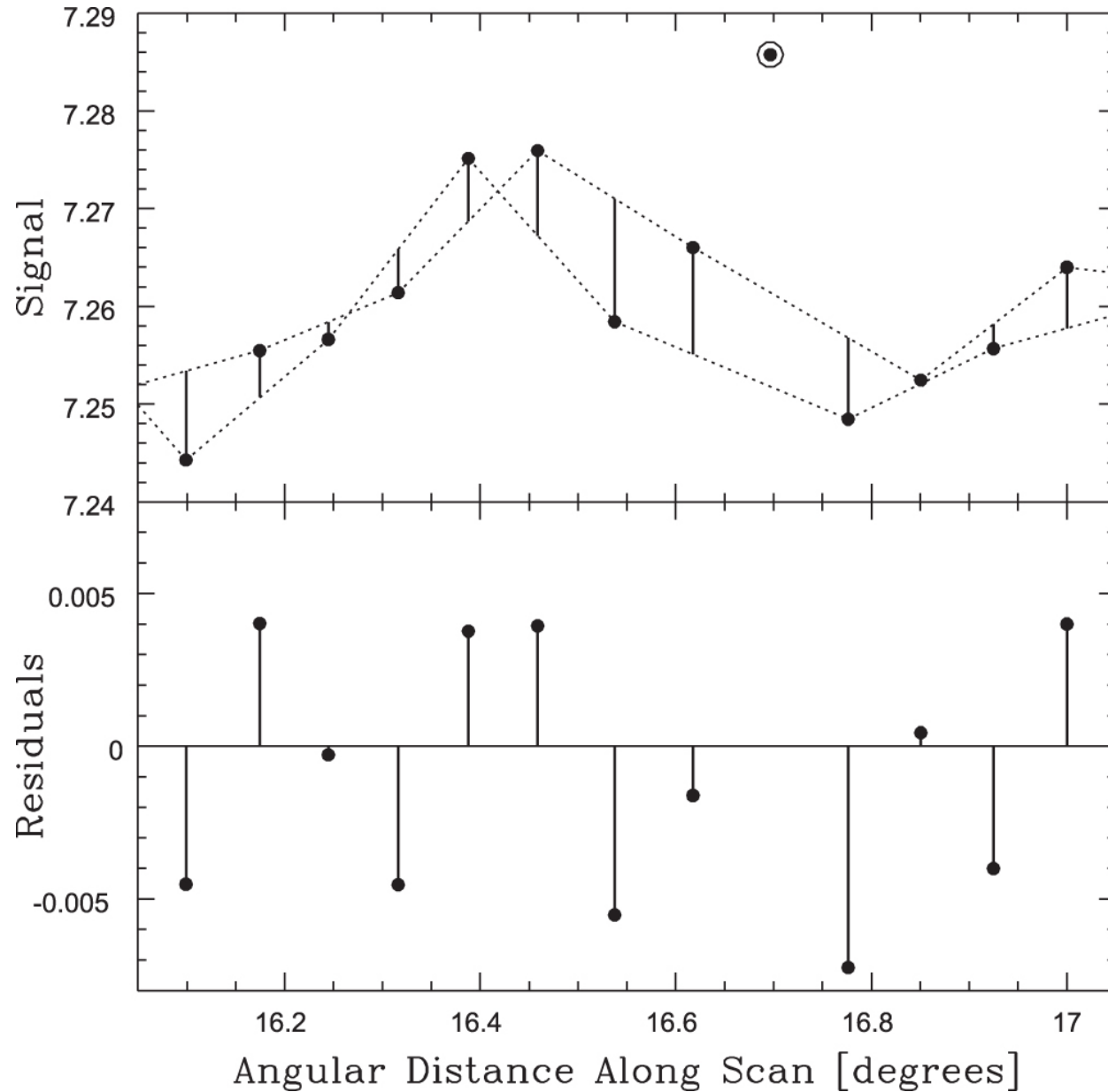
Figure 9. from Skynet Algorithm for Single-dish Radio Mapping. I. Contaminant-cleaning, Mapping, and Photometering Small-scale Structures null 2019 APJS 240 12 doi:10.3847/1538-4365/aad7c1 https://dx.doi.org/10.3847/1538-4365/aad7c1 © 2019. The American Astronomical Society. All rights reserved.
