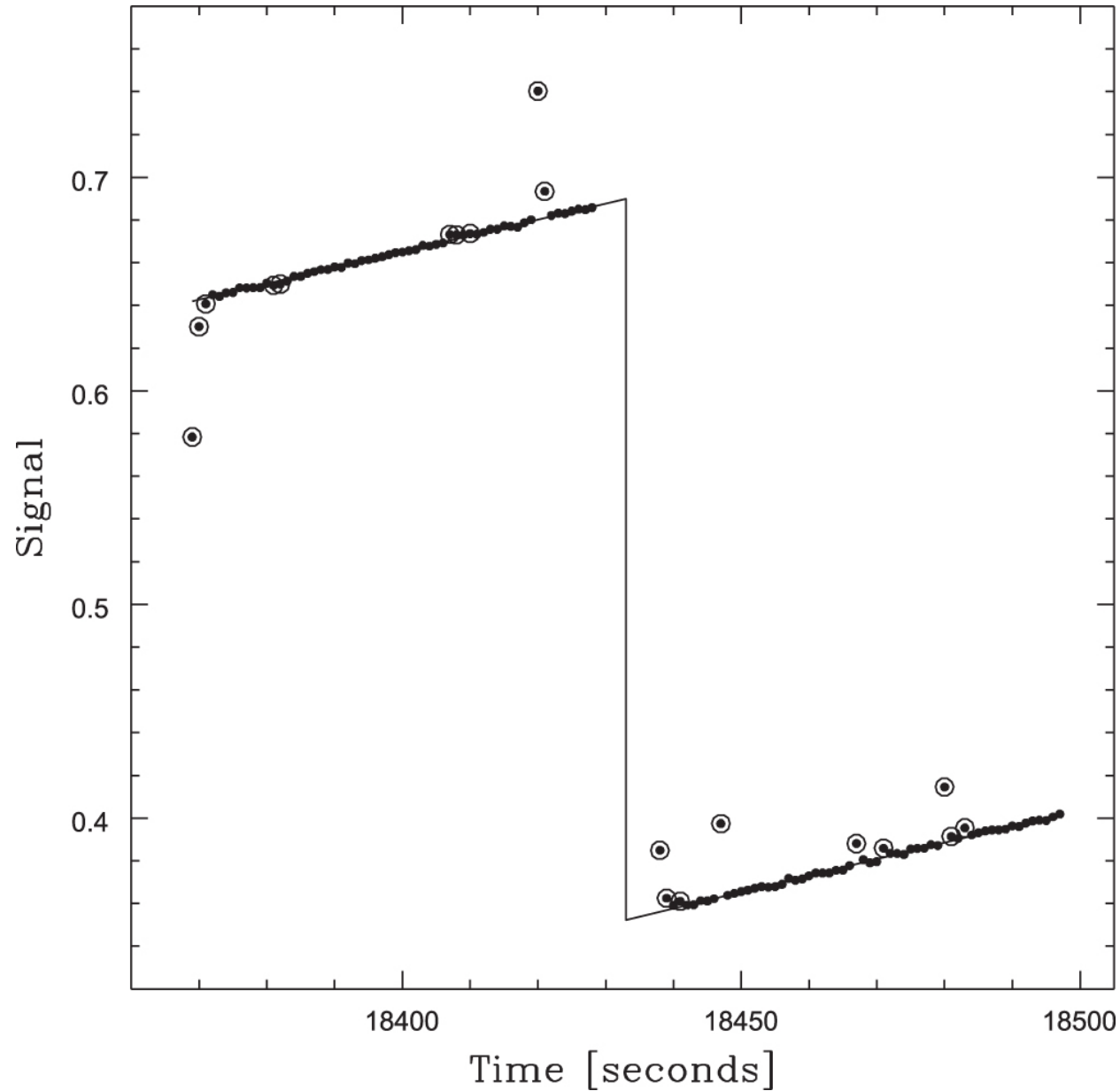
Figure 8. from Skynet Algorithm for Single-dish Radio Mapping. I. Contaminant-cleaning, Mapping, and Photometering Small-scale Structures null 2019 APJS 240 12 doi:10.3847/1538-4365/aad7c1 https://dx.doi.org/10.3847/1538-4365/aad7c1 © 2019. The American Astronomical Society. All rights reserved.
