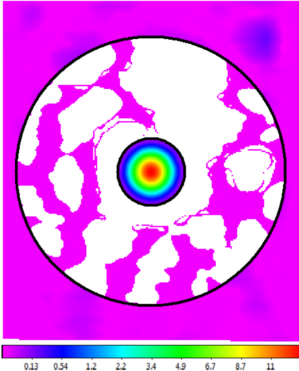
Figure 54. from Skynet Algorithm for Single-dish Radio Mapping. I. Contaminant-cleaning, Mapping, and Photometering Small-scale Structures null 2019 APJS 240 12 doi:10.3847/1538-4365/aad7c1 https://dx.doi.org/10.3847/1538-4365/aad7c1 © 2019. The American Astronomical Society. All rights reserved.
