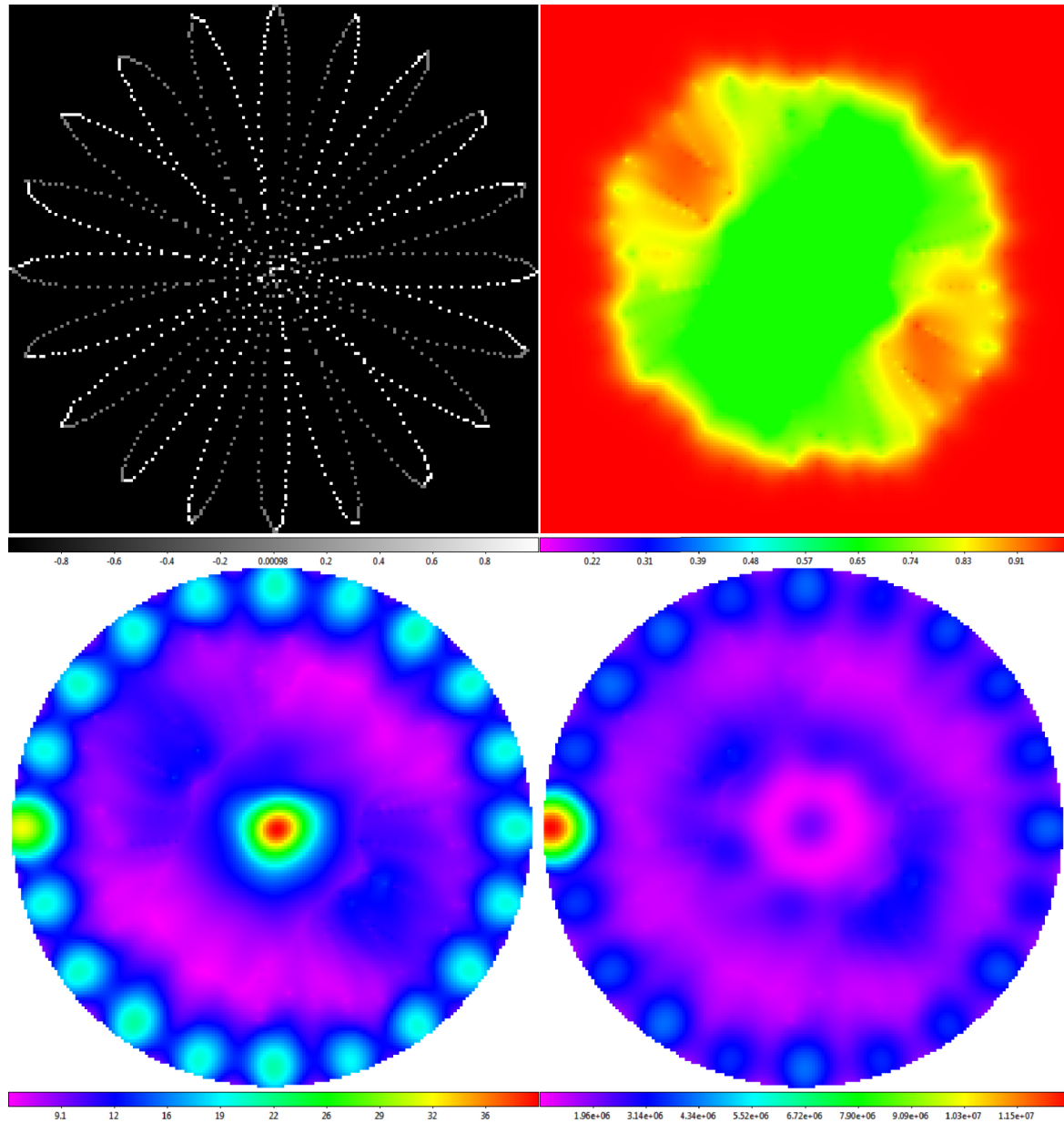
Figure 53. from Skynet Algorithm for Single-dish Radio Mapping. I. Contaminant-cleaning, Mapping, and Photometering Small-scale Structures null 2019 APJS 240 12 doi:10.3847/1538-4365/aad7c1 https://dx.doi.org/10.3847/1538-4365/aad7c1 © 2019. The American Astronomical Society. All rights reserved.
