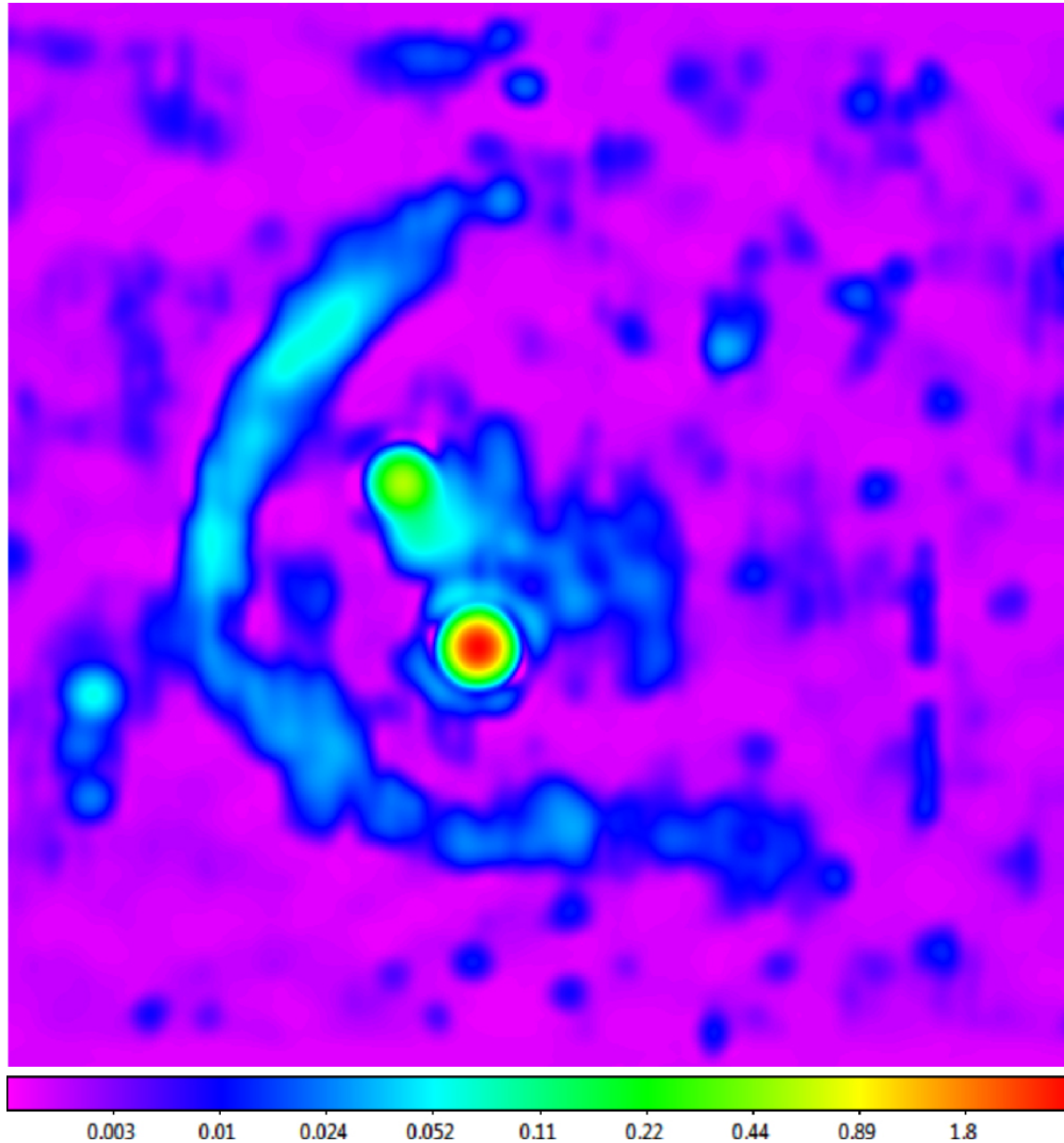
Figure 52. from Skynet Algorithm for Single-dish Radio Mapping. I. Contaminant-cleaning, Mapping, and Photometering Small-scale Structures null 2019 APJS 240 12 doi:10.3847/1538-4365/aad7c1 https://dx.doi.org/10.3847/1538-4365/aad7c1 © 2019. The American Astronomical Society. All rights reserved.
