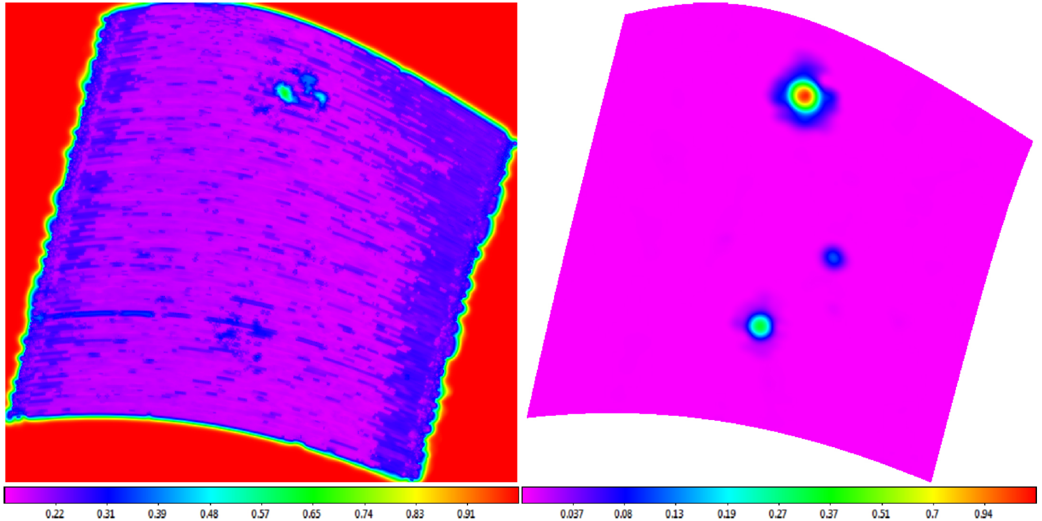
Figure 50. from Skynet Algorithm for Single-dish Radio Mapping. I. Contaminant-cleaning, Mapping, and Photometering Small-scale Structures null 2019 APJS 240 12 doi:10.3847/1538-4365/aad7c1 https://dx.doi.org/10.3847/1538-4365/aad7c1 © 2019. The American Astronomical Society. All rights reserved.
